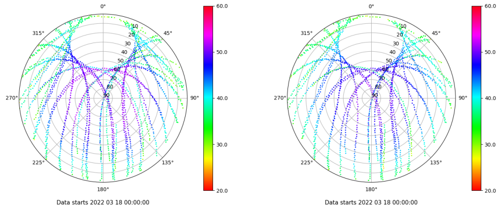
Skyplot for station VIGO. Signal to Noise S1C Data file VIGO00ESP_R_2022077.xtr Skyplot for station VIGO. Signal to Noise S2C Data file VIGO00ESP_R_2022077.xtr
