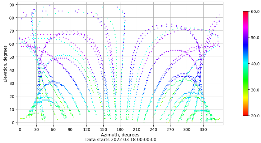
Azimuth-elevation plot for station VIGO. Signal to Noise S1C Data file VIGO00ESP_R_2022077.xtr
