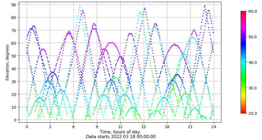
Time-elevation plot for station VIGO. Signal to Noise S1C Data file VIGO00ESP_R_2022077.xtr
