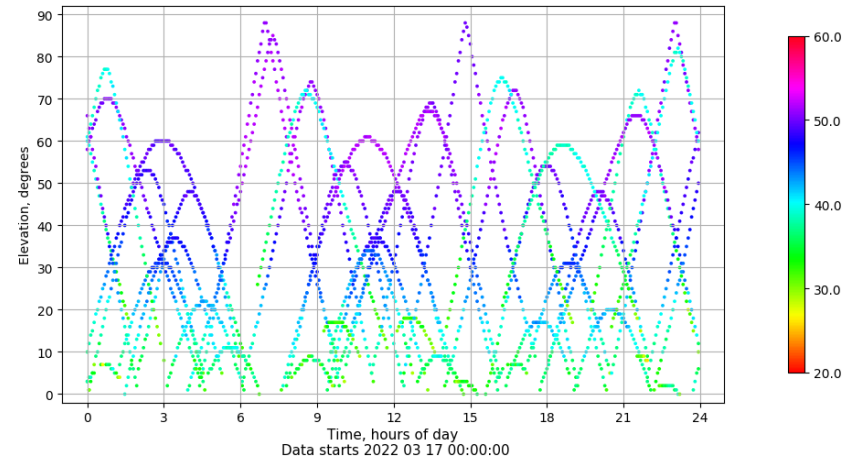
Time-elevation plot for station VIGO. Signal to Noise S1C Data file VIGO00ESP_R_2022076.xtr
