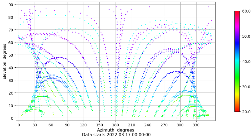
Azimuth-elevation plot for station VIGO. Signal to Noise S1C Data file VIGO00ESP_R_2022076.xtr
