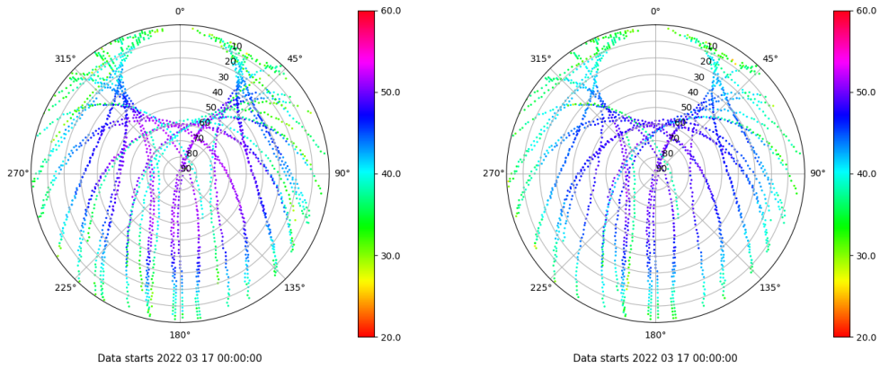
Skyplot for station VIGO. Signal to Noise S1C Data file VIGO00ESP_R_2022076.xtr Skyplot for station VIGO. Signal to Noise S2C Data file VIGO00ESP_R_2022076.xtr
