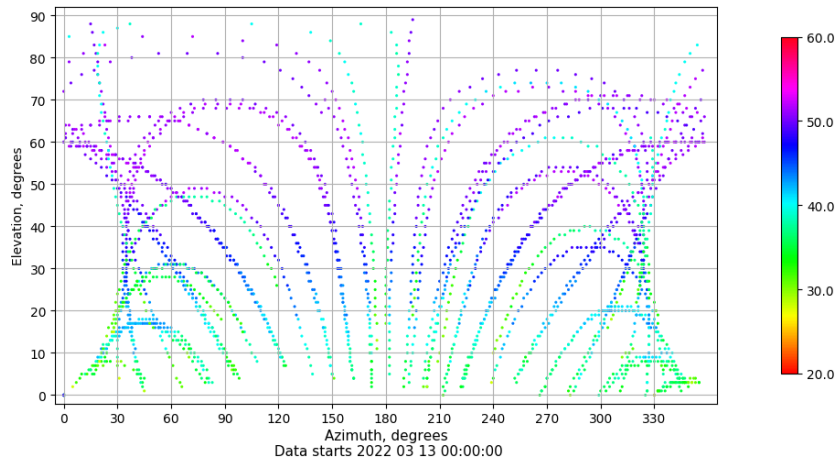
Azimuth-elevation plot for station VIGO. Signal to Noise S1C Data file VIGO00ESP_R_2022072.xtr
