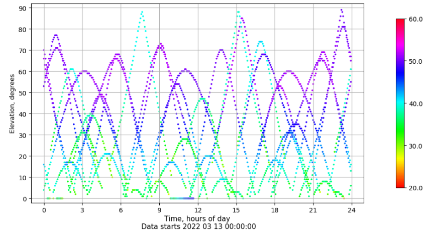
Time-elevation plot for station VIGO. Signal to Noise S1C Data file VIGO00ESP_R_2022072.xtr
