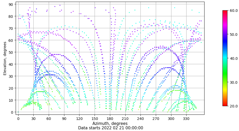
Azimuth-elevation plot for station VIGO. Signal to Noise S1C Data file VIGO00ESP_R_2022052.xtr
