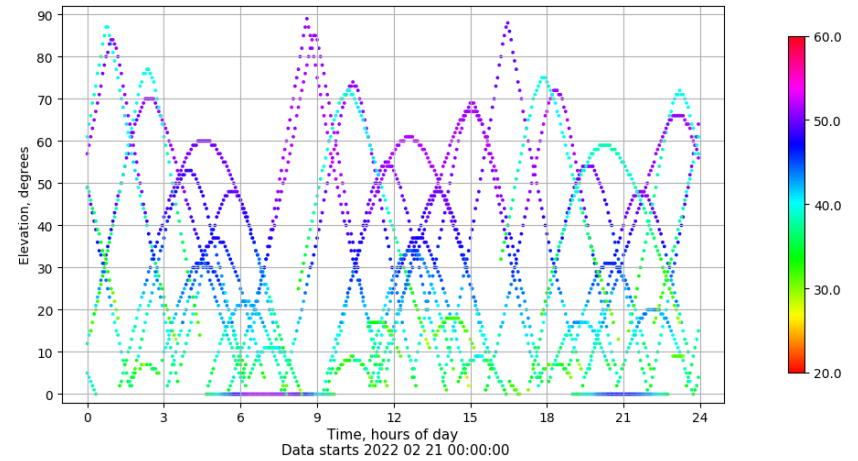
Time-elevation plot for station VIGO. Signal to Noise S1C Data file VIGO00ESP_R_2022052.xtr
