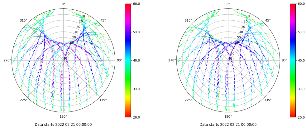
Skyplot for station VIGO. Signal to Noise S1C Data file VIGO00ESP_R_2022052.xtr Skyplot for station VIGO. Signal to Noise S2C Data file VIGO00ESP_R_2022052.xtr
