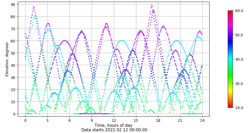
Time-elevation plot for station VIGO. Signal to Noise S1C Data file VIGO00ESP_R_2022043.xtr
