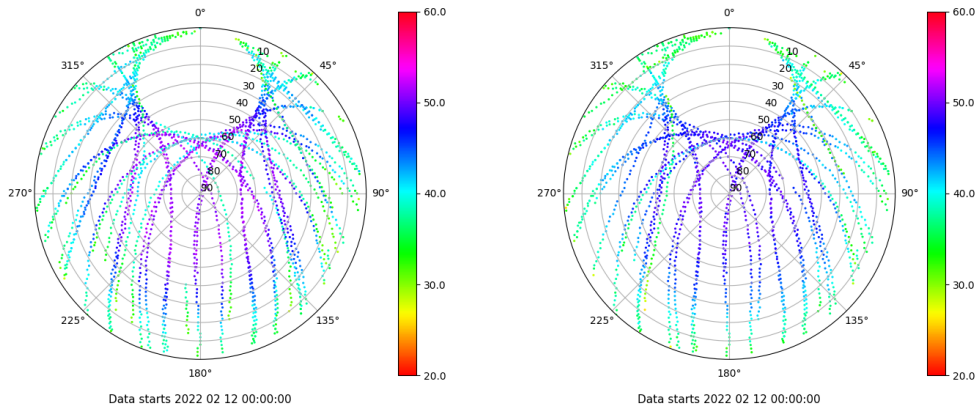
Skyplot for station VIGO. Signal to Noise S1C Data file VIGO00ESP_R_2022043.xtr Skyplot for station VIGO. Signal to Noise S2C Data file VIGO00ESP_R_2022043.xtr
