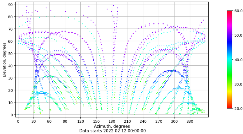
Azimuth-elevation plot for station VIGO. Signal to Noise S1C Data file VIGO00ESP_R_2022043.xtr
