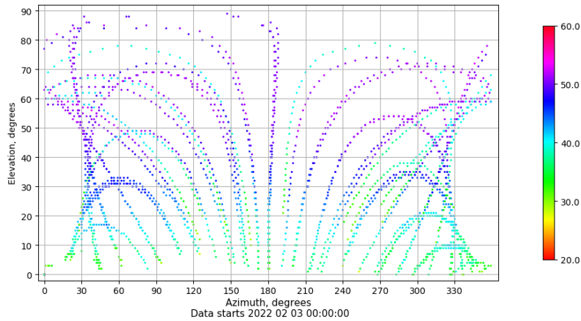
Azimuth-elevation plot for station VIGO. Signal to Noise S1C Data file VIGO00ESP_R_2022034.xtr
