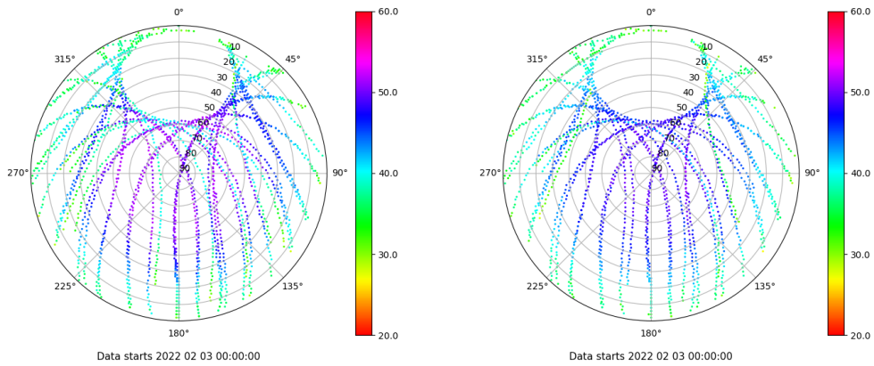
Skyplot for station VIGO. Signal to Noise S1C Data file VIGO00ESP_R_2022034.xtr Skyplot for station VIGO. Signal to Noise S2C Data file VIGO00ESP_R_2022034.xtr
