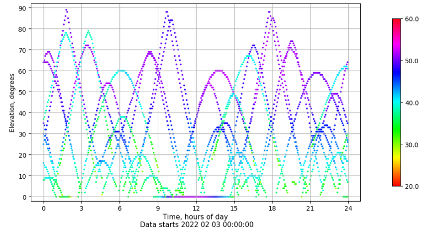
Time-elevation plot for station VIGO. Signal to Noise S1C Data file VIGO00ESP_R_2022034.xtr
