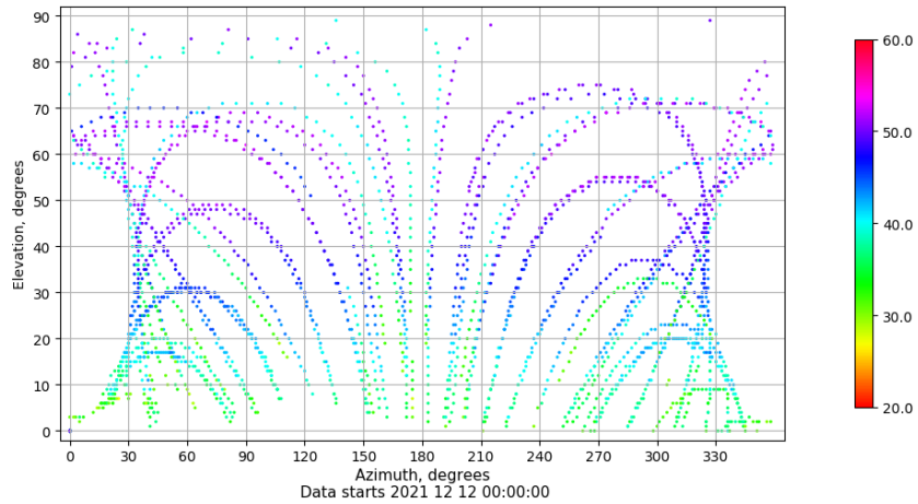
Azimuth-elevation plot for station VIGO. Signal to Noise S1C Data file VIGO00ESP_R_2021346.xtr
