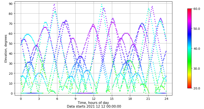
Time-elevation plot for station VIGO. Signal to Noise S1C Data file VIGO00ESP_R_2021346.xtr
