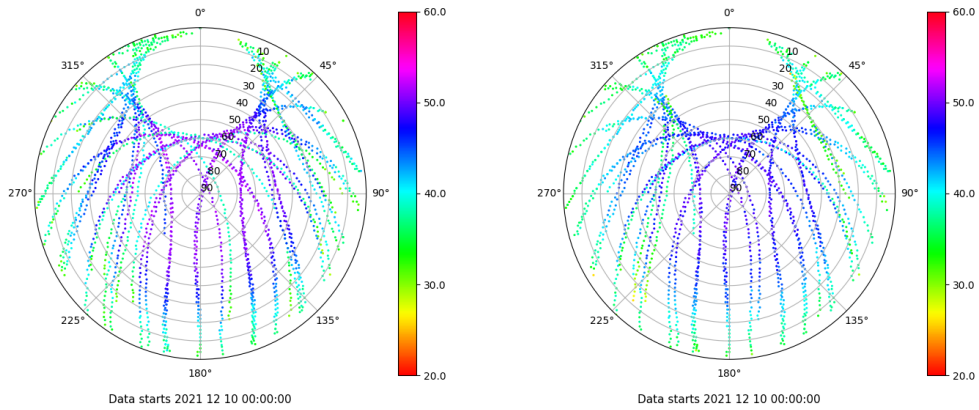
Skyplot for station VIGO. Signal to Noise S1C Data file VIGO00ESP_R_2021344.xtr Skyplot for station VIGO. Signal to Noise S2C Data file VIGO00ESP_R_2021344.xtr
