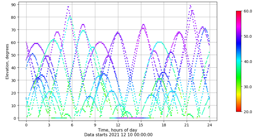
Time-elevation plot for station VIGO. Signal to Noise S1C Data file VIGO00ESP_R_2021344.xtr
