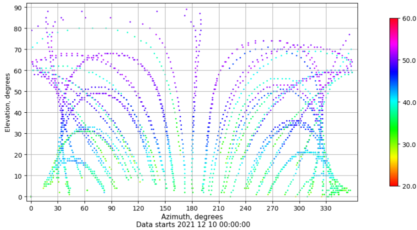
Azimuth-elevation plot for station VIGO. Signal to Noise S1C Data file VIGO00ESP_R_2021344.xtr
