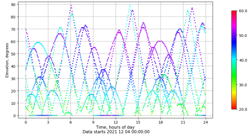
Time-elevation plot for station VIGO. Signal to Noise S1C Data file VIGO00ESP_R_2021338.xtr
