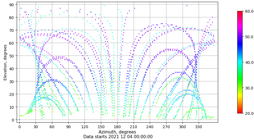
Azimuth-elevation plot for station VIGO. Signal to Noise S1C Data file VIGO00ESP_R_2021338.xtr
