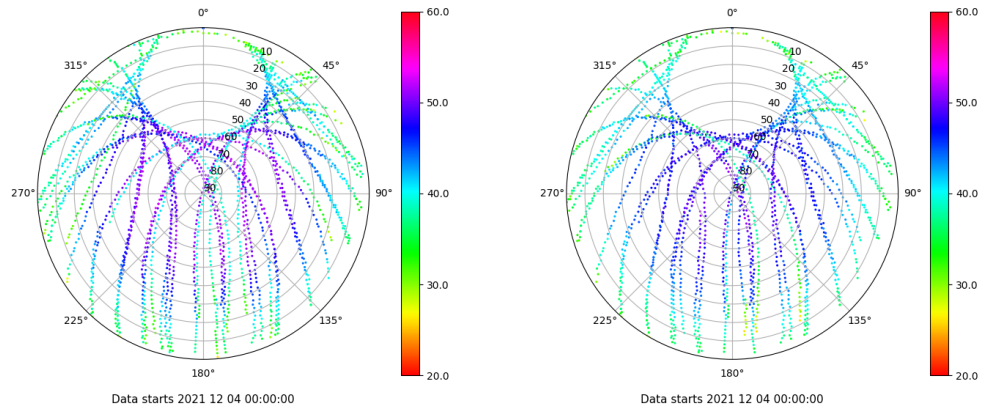
Skyplot for station VIGO. Signal to Noise S1C Data file VIGO00ESP_R_2021338.xtr Skyplot for station VIGO. Signal to Noise S2C Data file VIGO00ESP_R_2021338.xtr
