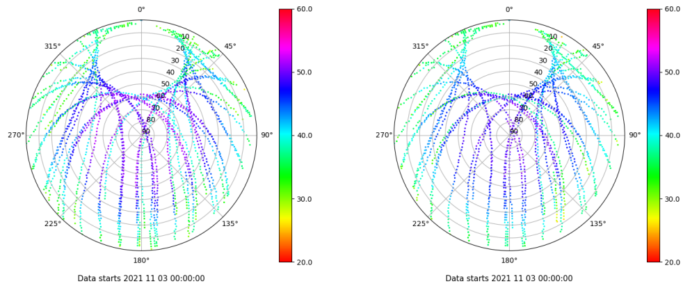
Skyplot for station VIGO. Signal to Noise S1C Data file VIGO00ESP_R_2021307.xtr Skyplot for station VIGO. Signal to Noise S2C Data file VIGO00ESP_R_2021307.xtr
