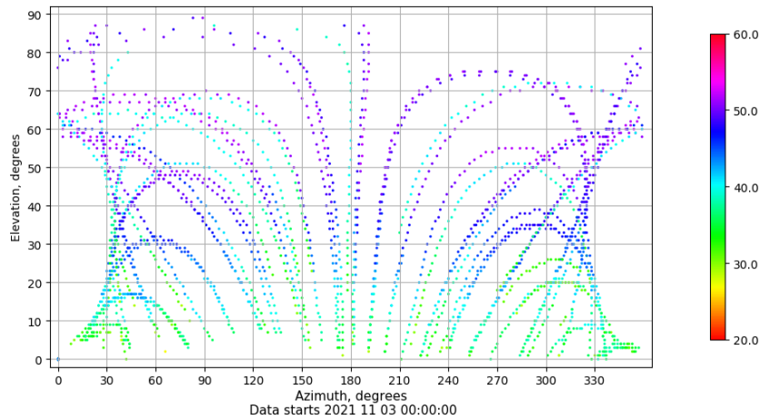
Azimuth-elevation plot for station VIGO. Signal to Noise S1C Data file VIGO00ESP_R_2021307.xtr
