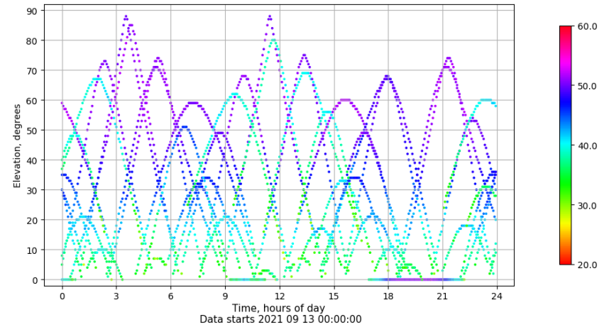
Time-elevation plot for station VIGO. Signal to Noise S1C Data file VIGO00ESP_R_2021256.xtr
