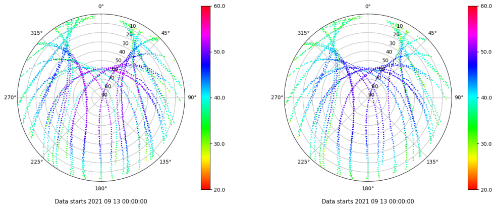
Skyplot for station VIGO. Signal to Noise S1C Data file VIGO00ESP_R_2021256.xtr Skyplot for station VIGO. Signal to Noise S2C Data file VIGO00ESP_R_2021256.xtr
