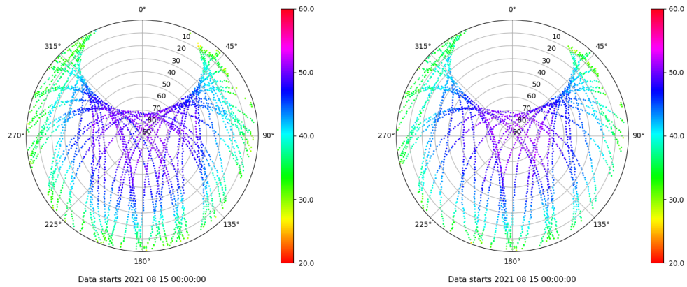
Skyplot for station VIGO. Signal to Noise S1C Data file VIGO00ESP_R_2021227.xtr Skyplot for station VIGO. Signal to Noise S2X Data file VIGO00ESP_R_2021227.xtr
