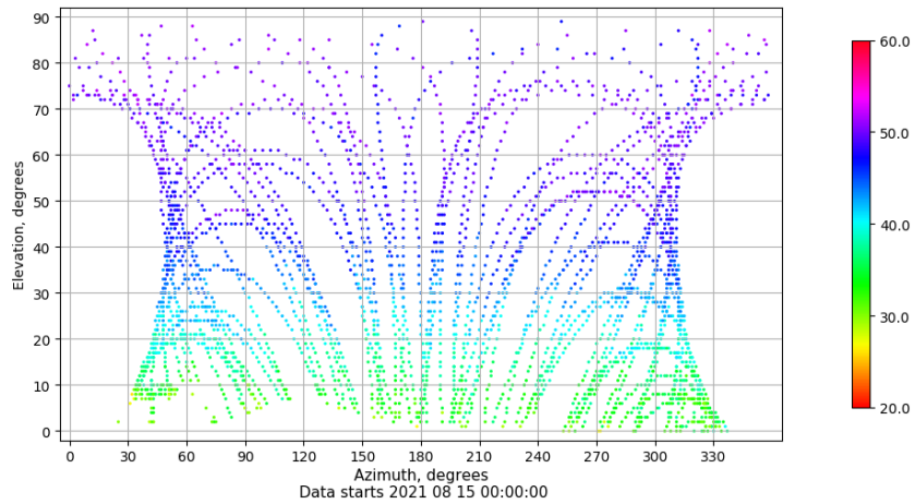
Azimuth-elevation plot for station VIGO. Signal to Noise S1C Data file VIGO00ESP_R_2021227.xtr
