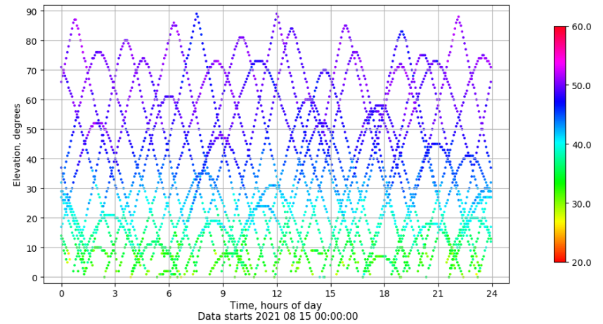
Time-elevation plot for station VIGO. Signal to Noise S1C Data file VIGO00ESP_R_2021227.xtr
