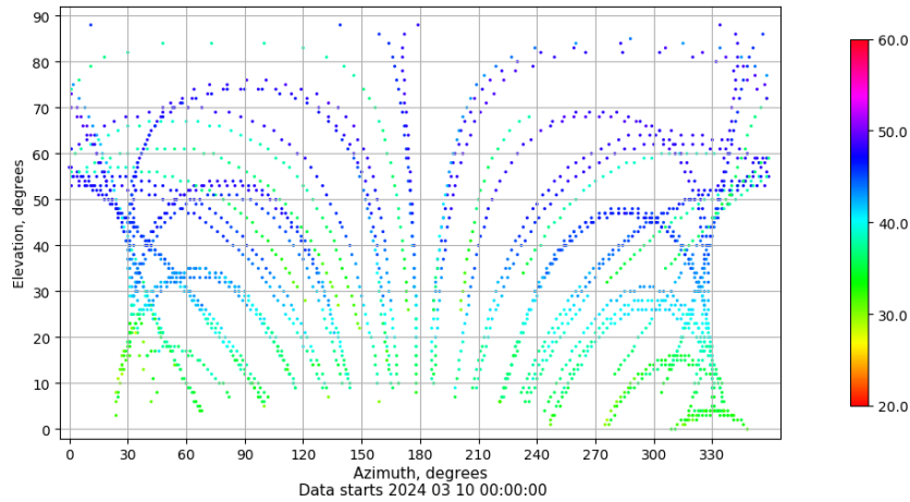
Azimuth-elevation plot for station VICA. Signal to Noise S1C Data file VICA00ESP_R_2024070.xtr
