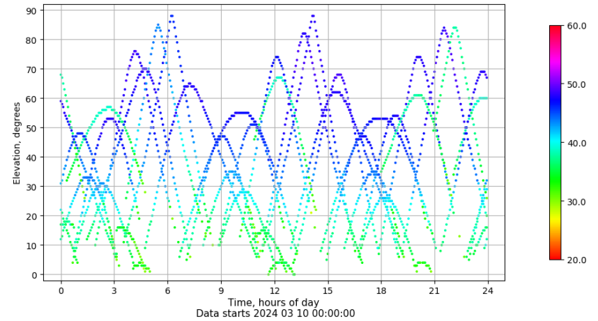
Time-elevation plot for station VICA. Signal to Noise S1C Data file VICA00ESP_R_2024070.xtr
