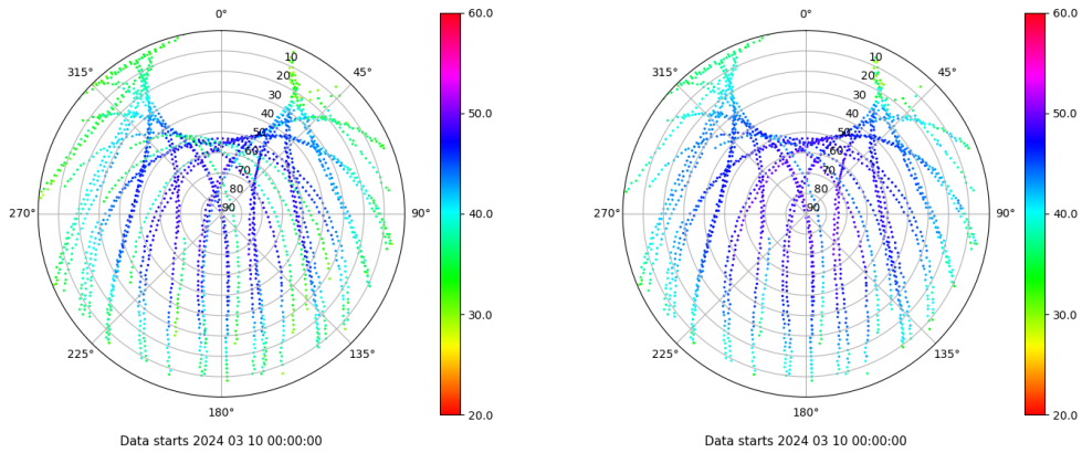
Skyplot for station VICA. Signal to Noise S1C Data file VICA00ESP_R_2024070.xtr Skyplot for station VICA. Signal to Noise S2P Data file VICA00ESP_R_2024070.xtr
