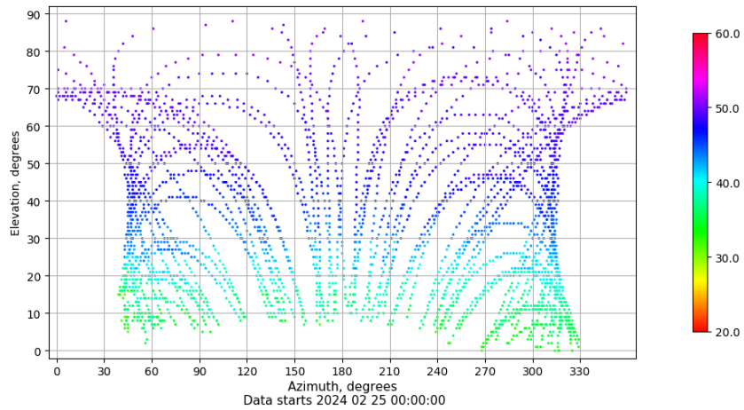
Azimuth-elevation plot for station VICA. Signal to Noise S1C Data file VICA00ESP_R_2024056.xtr
