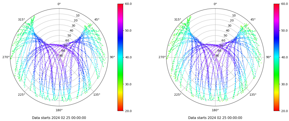
Skyplot for station VICA. Signal to Noise S1C Data file VICA00ESP_R_2024056.xtr Skyplot for station VICA. Signal to Noise S2W Data file VICA00ESP_R_2024056.xtr
