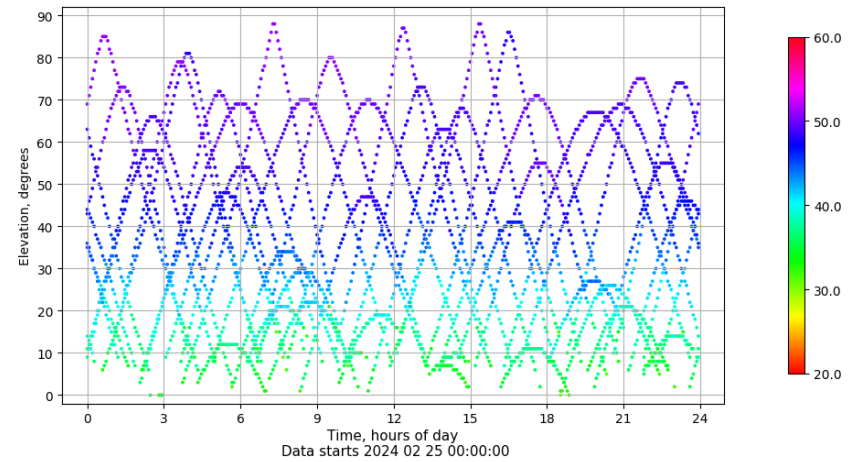
Time-elevation plot for station VICA. Signal to Noise S1C Data file VICA00ESP_R_2024056.xtr
