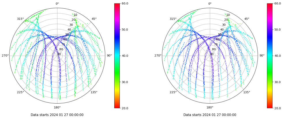
Skyplot for station VICA. Signal to Noise S1C Data file VICA00ESP_R_2024027.xtr Skyplot for station VICA. Signal to Noise S2P Data file VICA00ESP_R_2024027.xtr
