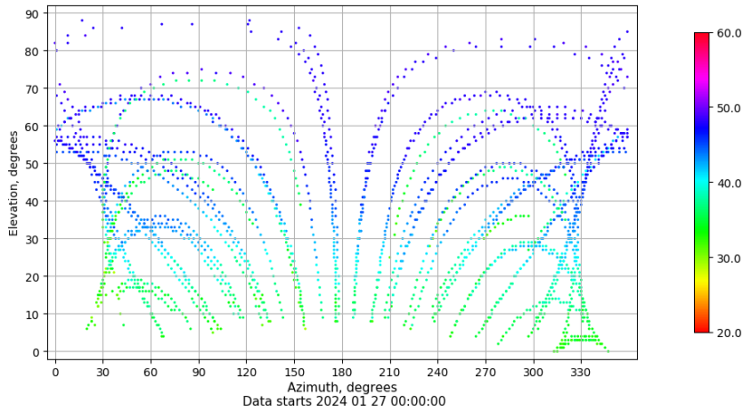
Azimuth-elevation plot for station VICA. Signal to Noise S1C Data file VICA00ESP_R_2024027.xtr
