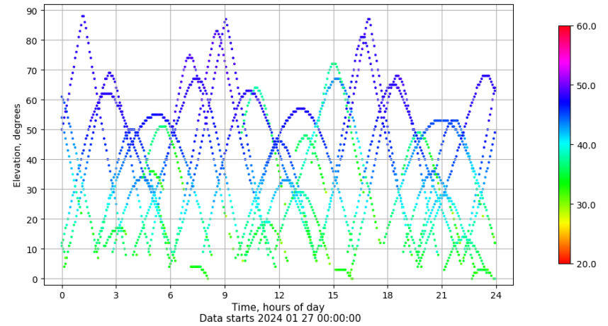
Time-elevation plot for station VICA. Signal to Noise S1C Data file VICA00ESP_R_2024027.xtr
