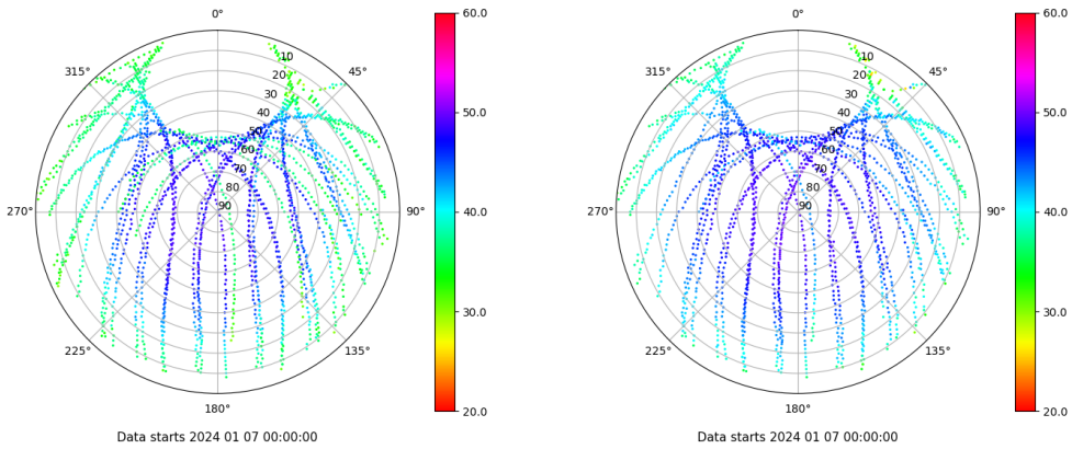
Skyplot for station VICA. Signal to Noise S1C Data file VICA00ESP_R_2024007.xtr Skyplot for station VICA. Signal to Noise S2P Data file VICA00ESP_R_2024007.xtr
