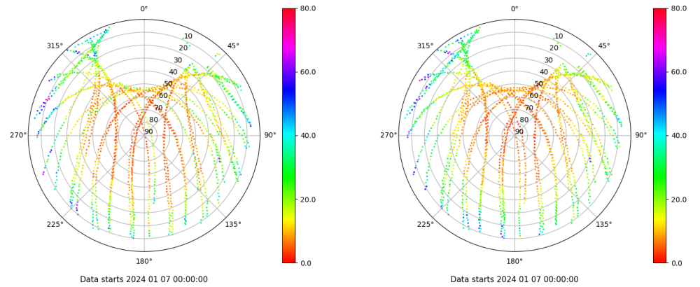
Skyplot for station VICA. Parameter M1C Data file VICA00ESP_R_2024007.xtr Skyplot for station VICA. Parameter M2P Data file VICA00ESP_R_2024007.xtr
