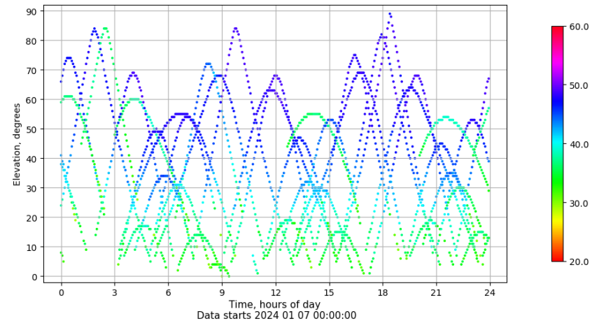
Time-elevation plot for station VICA. Signal to Noise S1C Data file VICA00ESP_R_2024007.xtr
