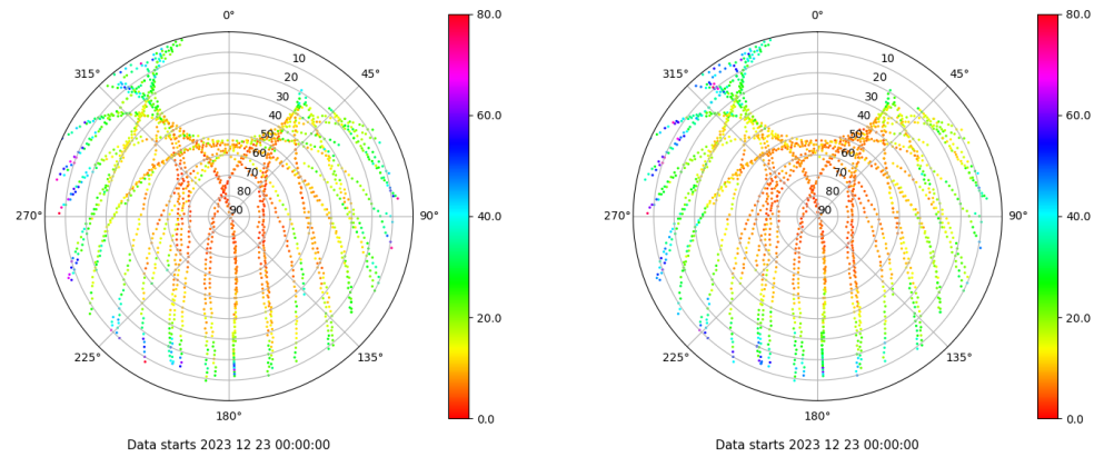
Skyplot for station VICA. Parameter M1C Data file VICA00ESP_R_2023357.xtr Skyplot for station VICA. Parameter M2P Data file VICA00ESP_R_2023357.xtr
