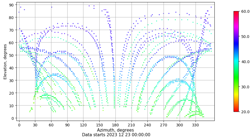
Azimuth-elevation plot for station VICA. Signal to Noise S1C Data file VICA00ESP_R_2023357.xtr
