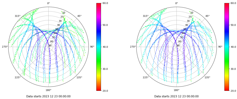
Skyplot for station VICA. Signal to Noise S1C Data file VICA00ESP_R_2023357.xtr Skyplot for station VICA. Signal to Noise S2P Data file VICA00ESP_R_2023357.xtr
