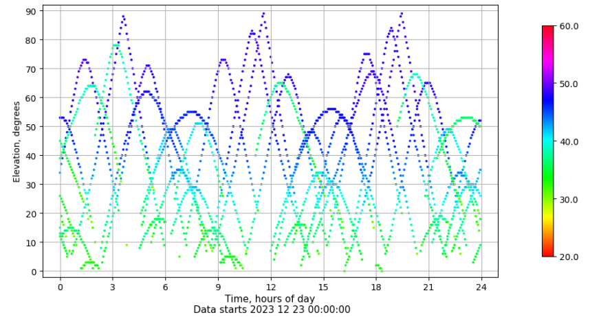
Time-elevation plot for station VICA. Signal to Noise S1C Data file VICA00ESP_R_2023357.xtr
