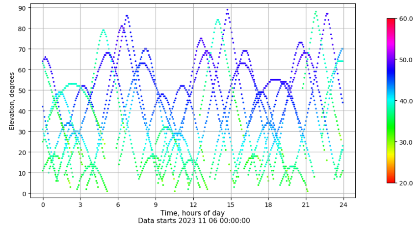
Time-elevation plot for station VICA. Signal to Noise S1C Data file VICA00ESP_R_2023310.xtr
