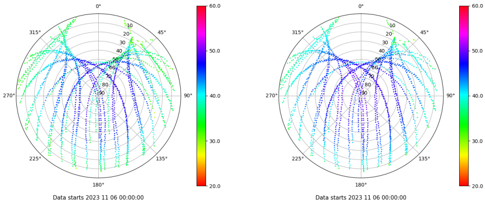
Skyplot for station VICA. Signal to Noise S1C Data file VICA00ESP_R_2023310.xtr Skyplot for station VICA. Signal to Noise S2P Data file VICA00ESP_R_2023310.xtr
