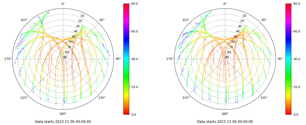
Skyplot for station VICA. Parameter M1C Data file VICA00ESP_R_2023310.xtr Skyplot for station VICA. Parameter M2P Data file VICA00ESP_R_2023310.xtr
