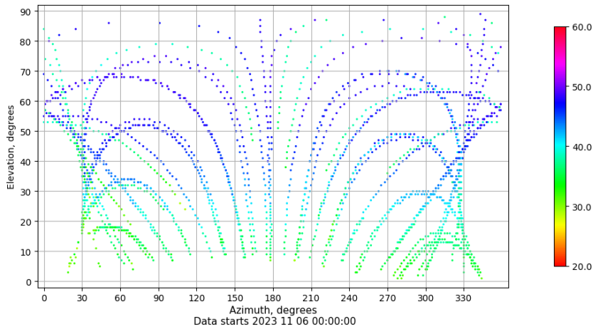
Azimuth-elevation plot for station VICA. Signal to Noise S1C Data file VICA00ESP_R_2023310.xtr
