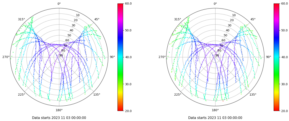
Skyplot for station VICA. Signal to Noise S1C Data file VICA00ESP_R_2023307.xtr Skyplot for station VICA. Signal to Noise S2W Data file VICA00ESP_R_2023307.xtr
