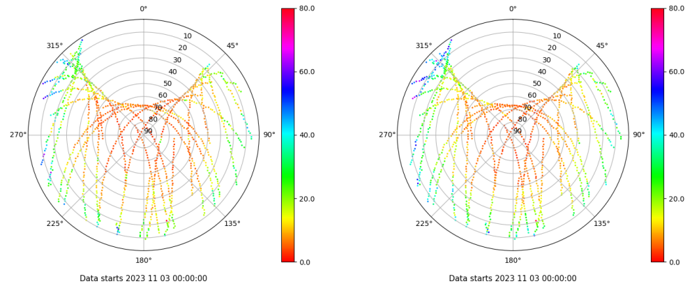
Skyplot for station VICA. Parameter M1C Data file VICA00ESP_R_2023307.xtr Skyplot for station VICA. Parameter M2W Data file VICA00ESP_R_2023307.xtr
