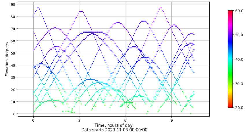
Time-elevation plot for station VICA. Signal to Noise S1C Data file VICA00ESP_R_2023307.xtr
