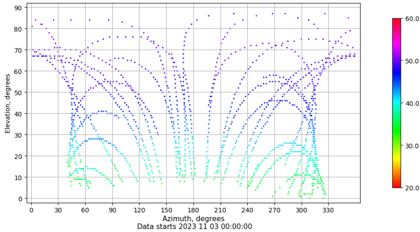
Azimuth-elevation plot for station VICA. Signal to Noise S1C Data file VICA00ESP_R_2023307.xtr
