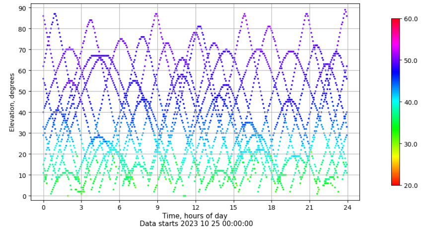
Time-elevation plot for station VICA. Signal to Noise S1C Data file VICA00ESP_R_2023298.xtr
