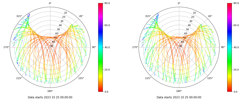
Skyplot for station VICA. Parameter M1C Data file VICA00ESP_R_2023298.xtr Skyplot for station VICA. Parameter M2W Data file VICA00ESP_R_2023298.xtr
