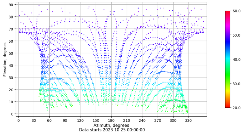
Azimuth-elevation plot for station VICA. Signal to Noise S1C Data file VICA00ESP_R_2023298.xtr
