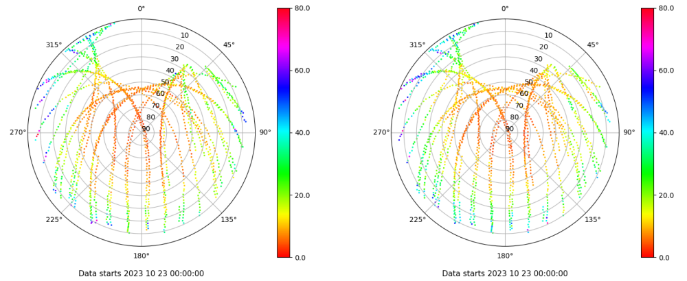
Skyplot for station VICA. Parameter M1C Data file VICA00ESP_R_2023296.xtr Skyplot for station VICA. Parameter M2P Data file VICA00ESP_R_2023296.xtr
