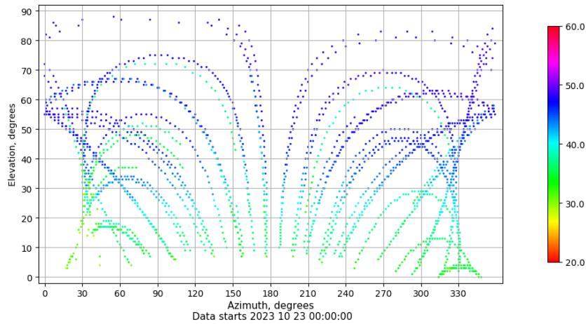
Azimuth-elevation plot for station VICA. Signal to Noise S1C Data file VICA00ESP_R_2023296.xtr
