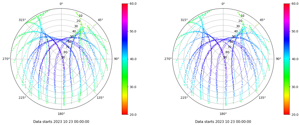
Skyplot for station VICA. Signal to Noise S1C Data file VICA00ESP_R_2023296.xtr Skyplot for station VICA. Signal to Noise S2P Data file VICA00ESP_R_2023296.xtr
