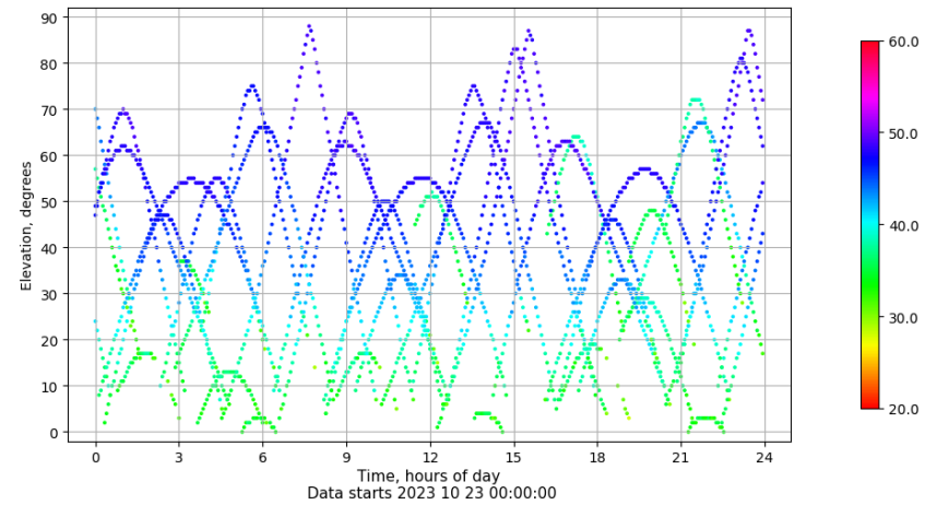
Time-elevation plot for station VICA. Signal to Noise S1C Data file VICA00ESP_R_2023296.xtr
