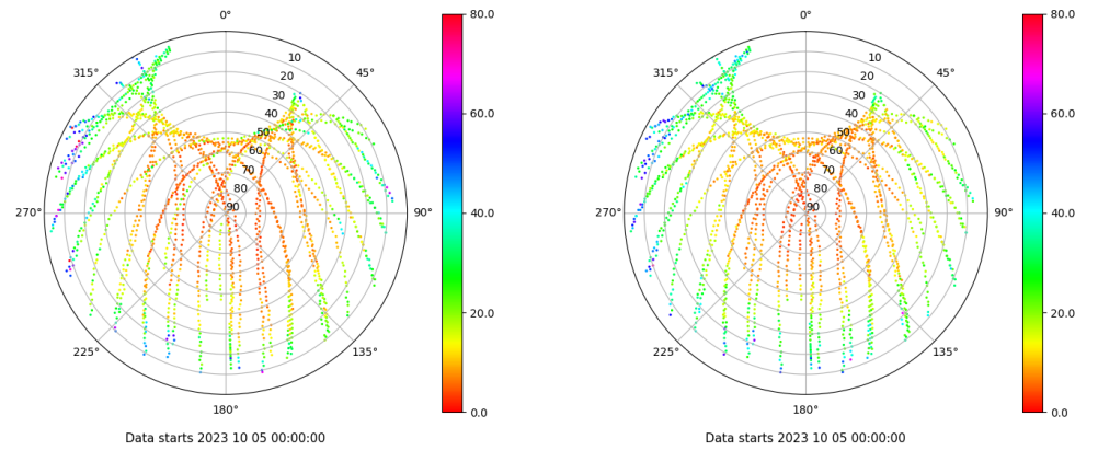
Skyplot for station VICA. Parameter M1C Data file VICA00ESP_R_2023278.xtr Skyplot for station VICA. Parameter M2P Data file VICA00ESP_R_2023278.xtr
