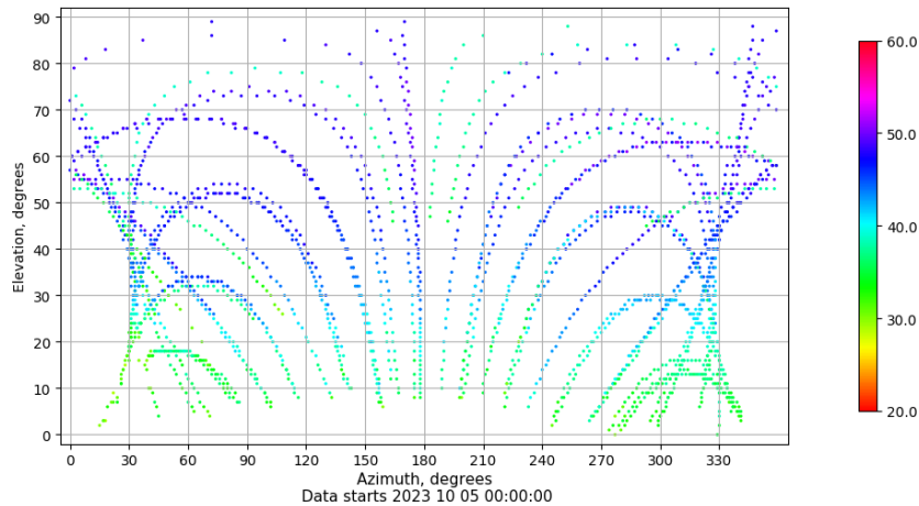
Azimuth-elevation plot for station VICA. Signal to Noise S1C Data file VICA00ESP_R_2023278.xtr
