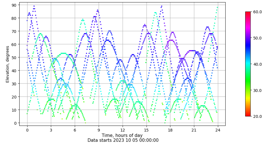
Time-elevation plot for station VICA. Signal to Noise S1C Data file VICA00ESP_R_2023278.xtr
