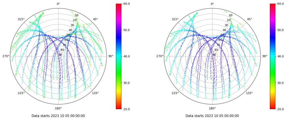
Skyplot for station VICA. Signal to Noise S1C Data file VICA00ESP_R_2023278.xtr Skyplot for station VICA. Signal to Noise S2P Data file VICA00ESP_R_2023278.xtr
