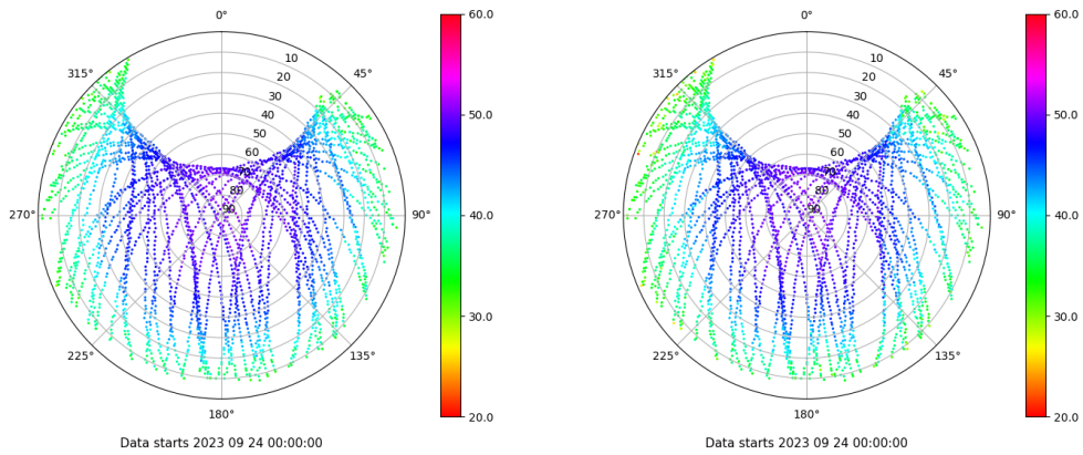
Skyplot for station VICA. Signal to Noise S1C Data file VICA00ESP_R_2023267.xtr Skyplot for station VICA. Signal to Noise S2W Data file VICA00ESP_R_2023267.xtr
