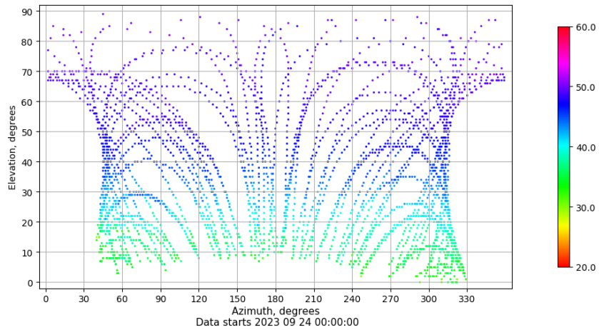
Azimuth-elevation plot for station VICA. Signal to Noise S1C Data file VICA00ESP_R_2023267.xtr
