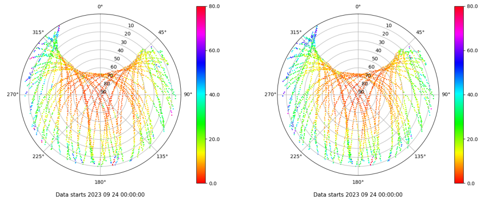
Skyplot for station VICA. Parameter M1C Data file VICA00ESP_R_2023267.xtr Skyplot for station VICA. Parameter M2W Data file VICA00ESP_R_2023267.xtr
