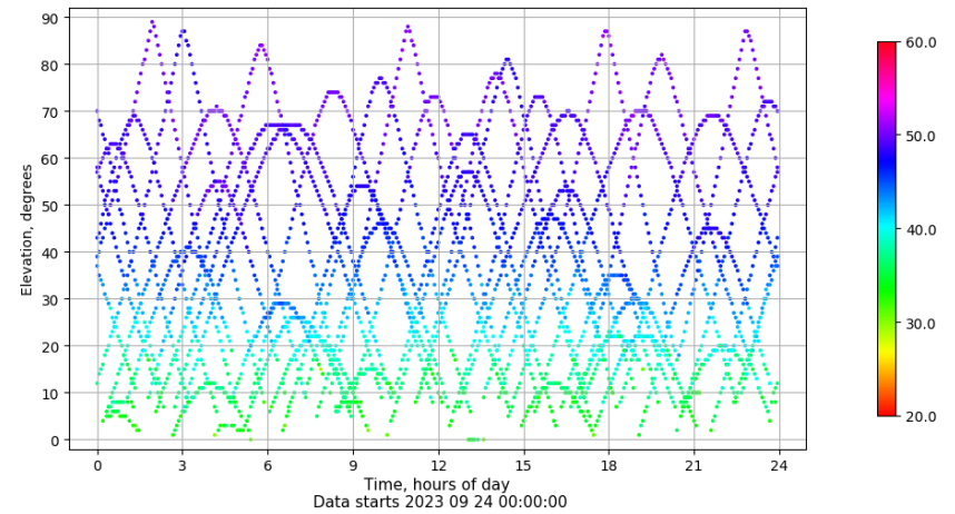
Time-elevation plot for station VICA. Signal to Noise S1C Data file VICA00ESP_R_2023267.xtr
