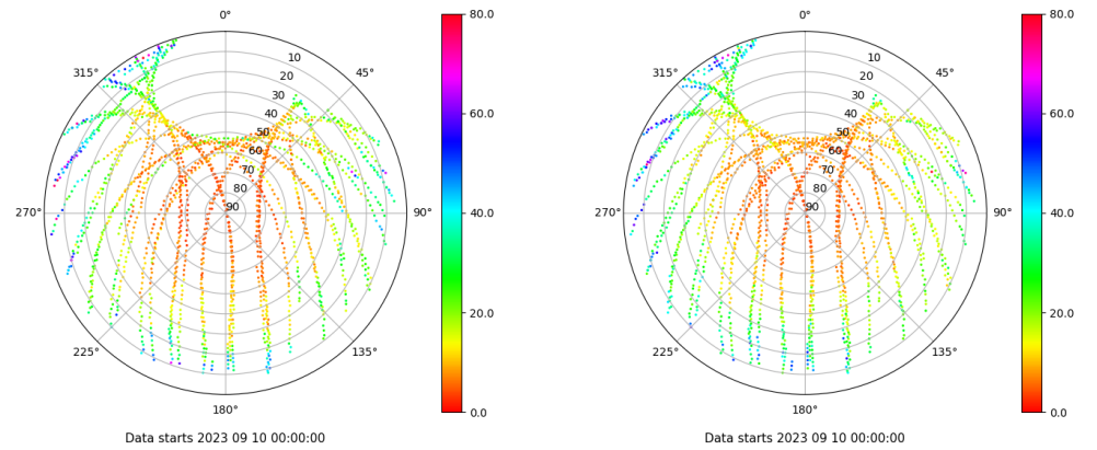
Skyplot for station VICA. Parameter M1C Data file VICA00ESP_R_2023253.xtr Skyplot for station VICA. Parameter M2P Data file VICA00ESP_R_2023253.xtr
