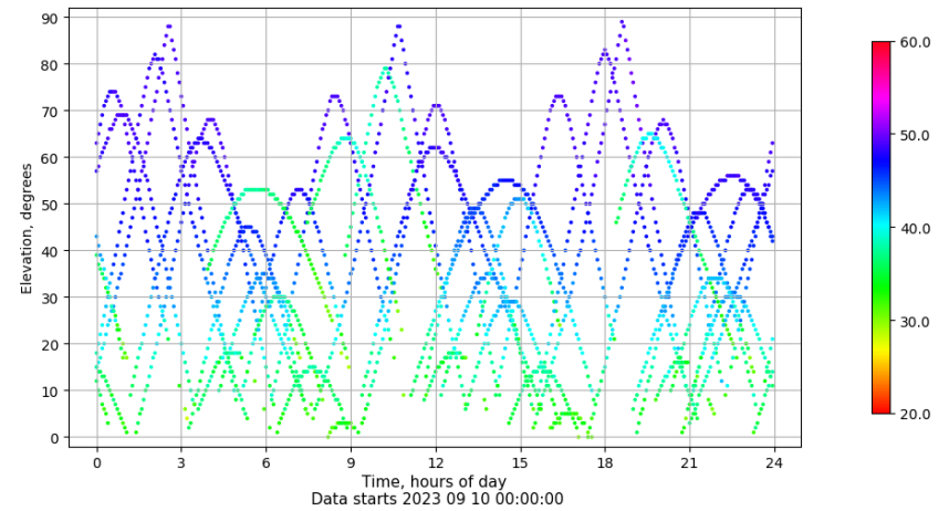
Time-elevation plot for station VICA. Signal to Noise S1C Data file VICA00ESP_R_2023253.xtr
