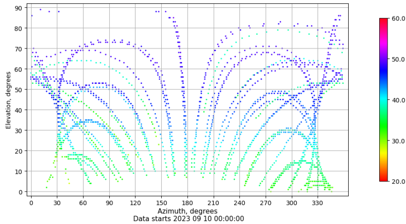
Azimuth-elevation plot for station VICA. Signal to Noise S1C Data file VICA00ESP_R_2023253.xtr
