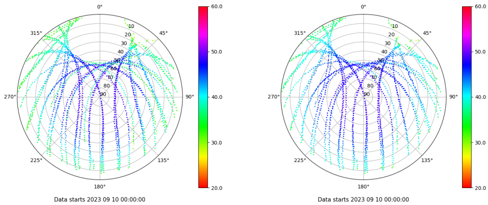
Skyplot for station VICA. Signal to Noise S1C Data file VICA00ESP_R_2023253.xtr Skyplot for station VICA. Signal to Noise S2P Data file VICA00ESP_R_2023253.xtr
