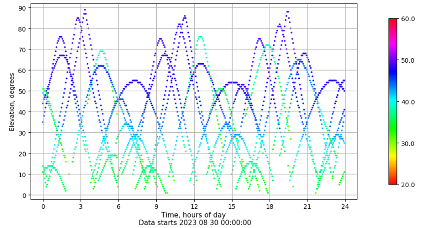
Time-elevation plot for station VICA. Signal to Noise S1C Data file VICA00ESP_R_2023242.xtr
