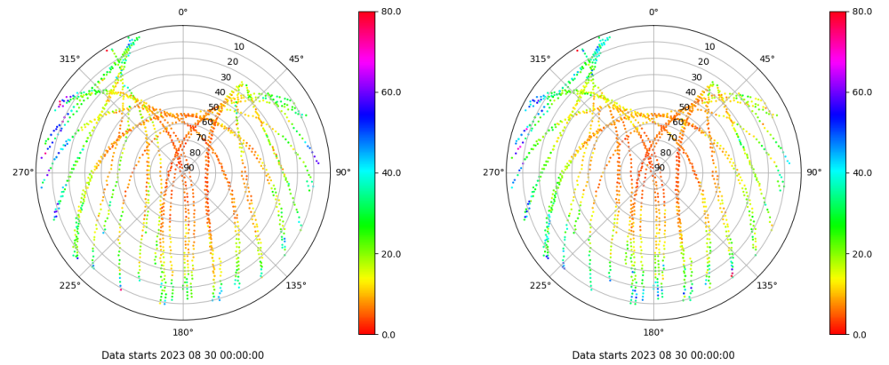
Skyplot for station VICA. Parameter M1C Data file VICA00ESP_R_2023242.xtr Skyplot for station VICA. Parameter M2P Data file VICA00ESP_R_2023242.xtr
