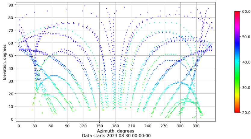
Azimuth-elevation plot for station VICA. Signal to Noise S1C Data file VICA00ESP_R_2023242.xtr
