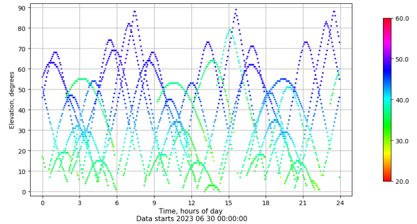
Time-elevation plot for station VICA. Signal to Noise S1C Data file VICA00ESP_R_2023181.xtr
