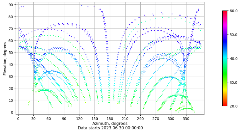
Azimuth-elevation plot for station VICA. Signal to Noise S1C Data file VICA00ESP_R_2023181.xtr
