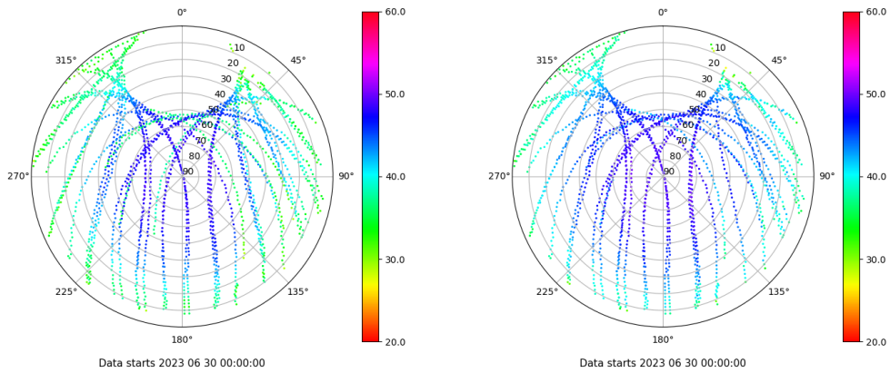
Skyplot for station VICA. Signal to Noise S1C Data file VICA00ESP_R_2023181.xtr Skyplot for station VICA. Signal to Noise S2P Data file VICA00ESP_R_2023181.xtr
