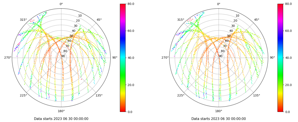
Skyplot for station VICA. Parameter M1C Data file VICA00ESP_R_2023181.xtr Skyplot for station VICA. Parameter M2P Data file VICA00ESP_R_2023181.xtr
