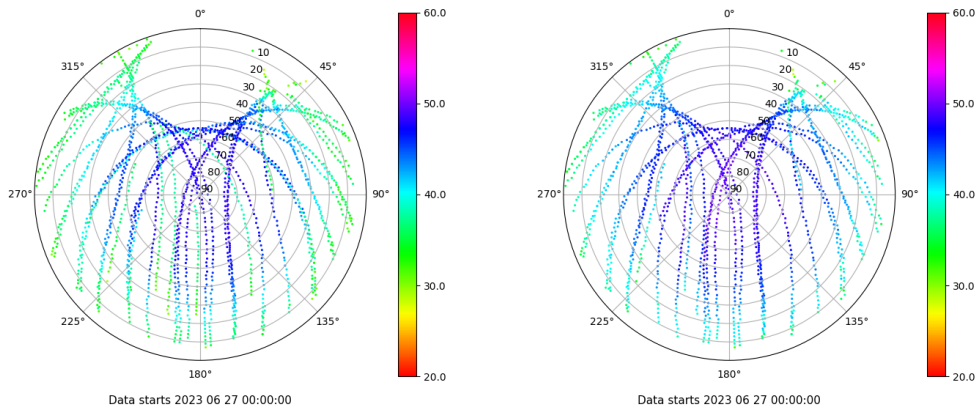
Skyplot for station VICA. Signal to Noise S1C Data file VICA00ESP_R_2023178.xtr Skyplot for station VICA. Signal to Noise S2P Data file VICA00ESP_R_2023178.xtr
