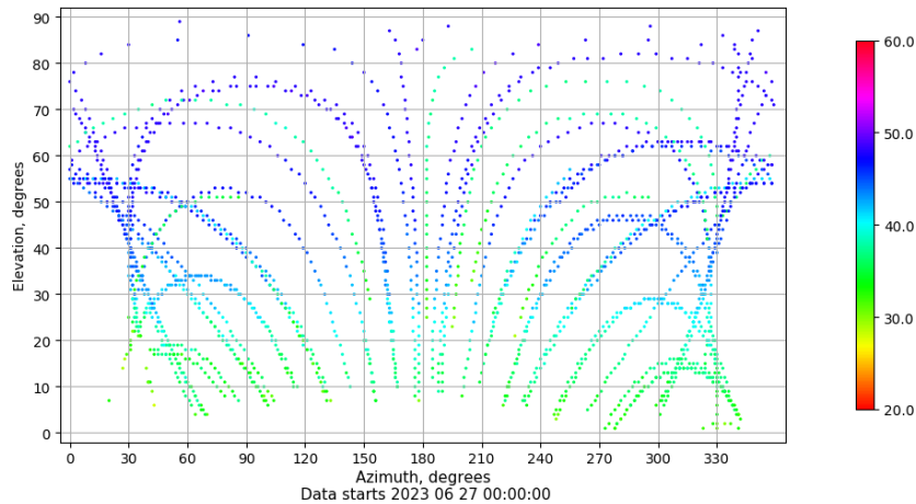
Azimuth-elevation plot for station VICA. Signal to Noise S1C Data file VICA00ESP_R_2023178.xtr
