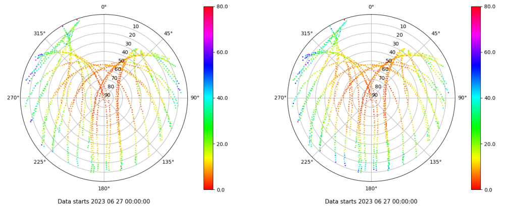
Skyplot for station VICA. Parameter M1C Data file VICA00ESP_R_2023178.xtr Skyplot for station VICA. Parameter M2P Data file VICA00ESP_R_2023178.xtr
