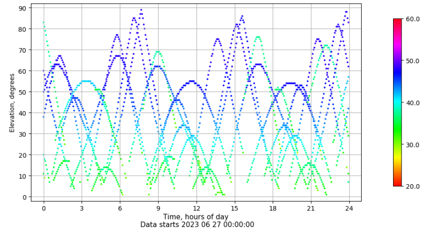
Time-elevation plot for station VICA. Signal to Noise S1C Data file VICA00ESP_R_2023178.xtr
