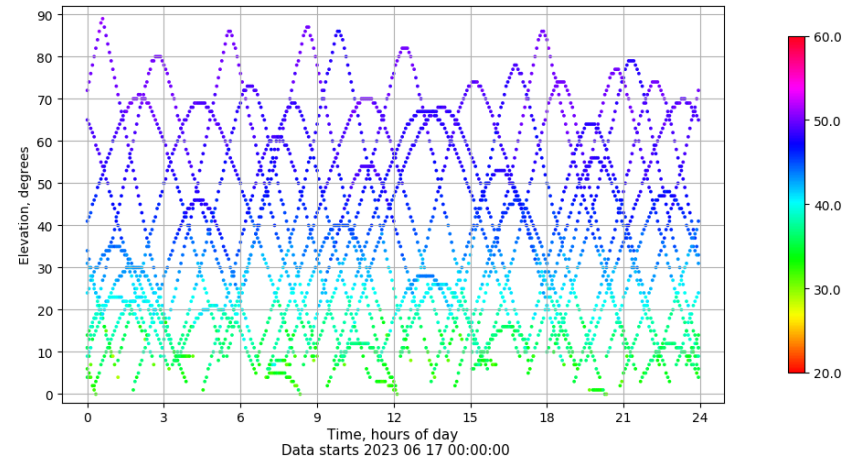
Time-elevation plot for station VICA. Signal to Noise S1C Data file VICA00ESP_R_2023168.xtr
