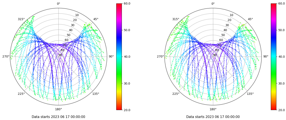
Skyplot for station VICA. Signal to Noise S1C Data file VICA00ESP_R_2023168.xtr Skyplot for station VICA. Signal to Noise S2W Data file VICA00ESP_R_2023168.xtr
