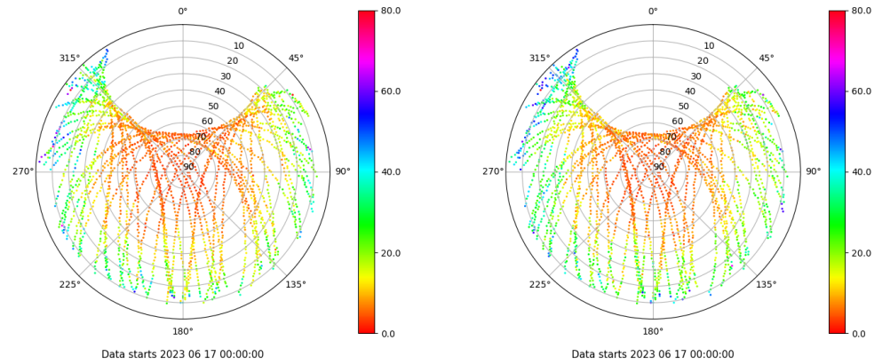
Skyplot for station VICA. Parameter M1C Data file VICA00ESP_R_2023168.xtr Skyplot for station VICA. Parameter M2W Data file VICA00ESP_R_2023168.xtr
