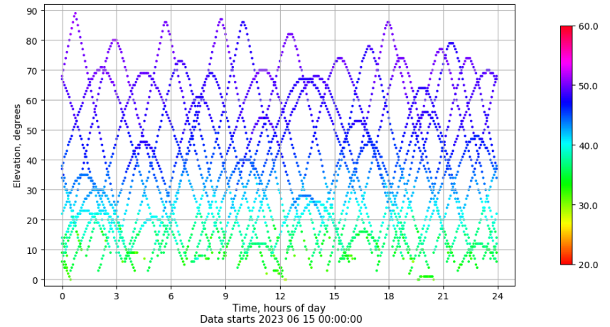
Time-elevation plot for station VICA. Signal to Noise S1C Data file VICA00ESP_R_2023166.xtr
