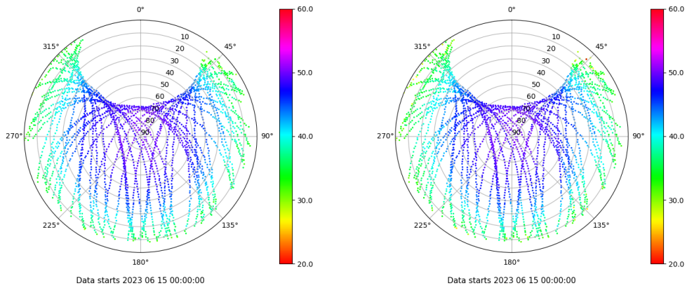
Skyplot for station VICA. Signal to Noise S1C Data file VICA00ESP_R_2023166.xtr Skyplot for station VICA. Signal to Noise S2W Data file VICA00ESP_R_2023166.xtr
