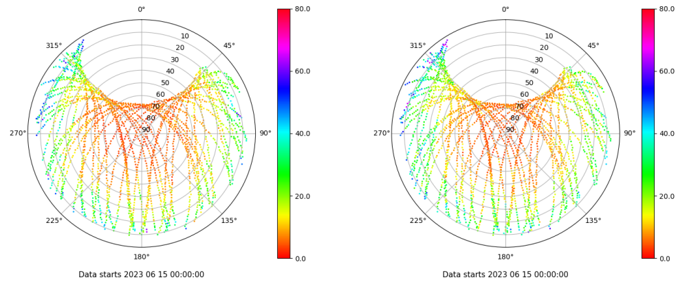
Skyplot for station VICA. Parameter M1C Data file VICA00ESP_R_2023166.xtr Skyplot for station VICA. Parameter M2W Data file VICA00ESP_R_2023166.xtr
