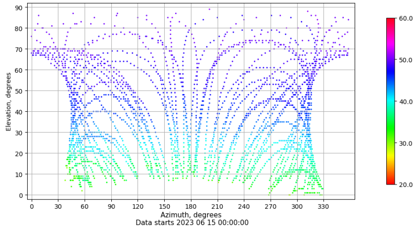
Azimuth-elevation plot for station VICA. Signal to Noise S1C Data file VICA00ESP_R_2023166.xtr
