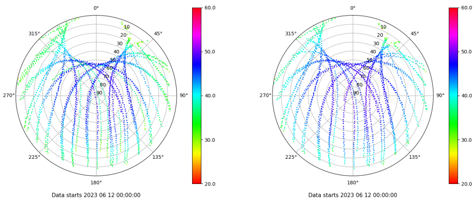
Skyplot for station VICA. Signal to Noise S1C Data file VICA00ESP_R_2023163.xtr Skyplot for station VICA. Signal to Noise S2P Data file VICA00ESP_R_2023163.xtr
