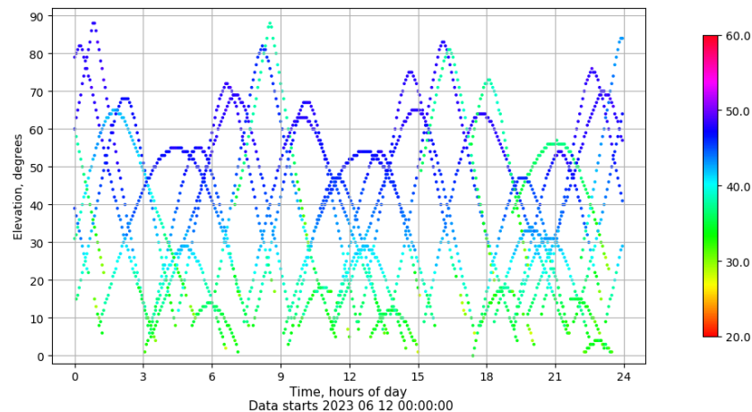
Time-elevation plot for station VICA. Signal to Noise S1C Data file VICA00ESP_R_2023163.xtr
