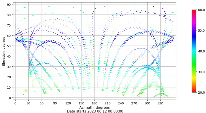
Azimuth-elevation plot for station VICA. Signal to Noise S1C Data file VICA00ESP_R_2023163.xtr
