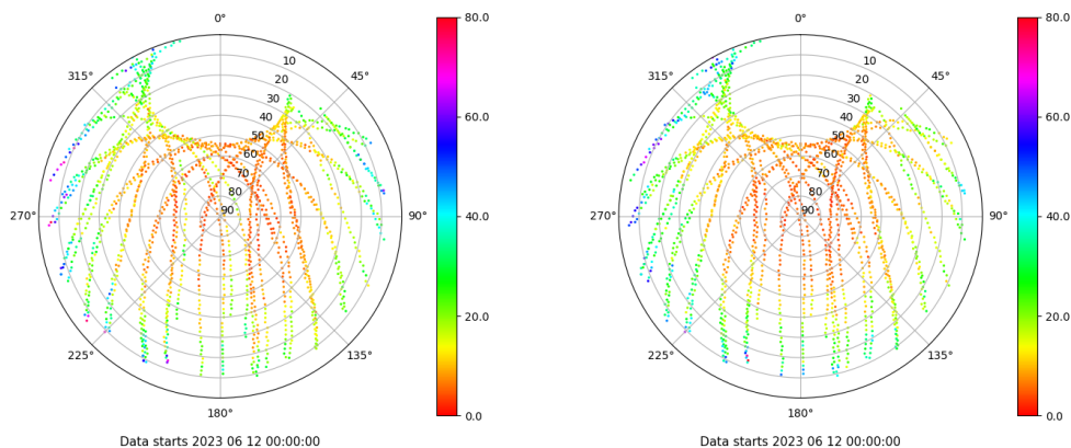
Skyplot for station VICA. Parameter M1C Data file VICA00ESP_R_2023163.xtr Skyplot for station VICA. Parameter M2P Data file VICA00ESP_R_2023163.xtr
