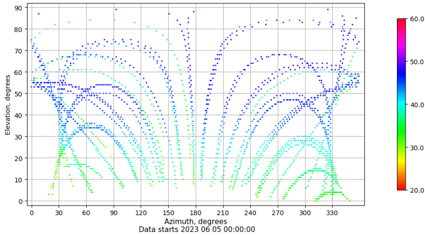
Azimuth-elevation plot for station VICA. Signal to Noise S1C Data file VICA00ESP_R_2023156.xtr
