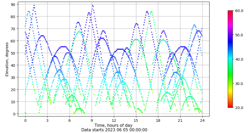
Time-elevation plot for station VICA. Signal to Noise S1C Data file VICA00ESP_R_2023156.xtr
