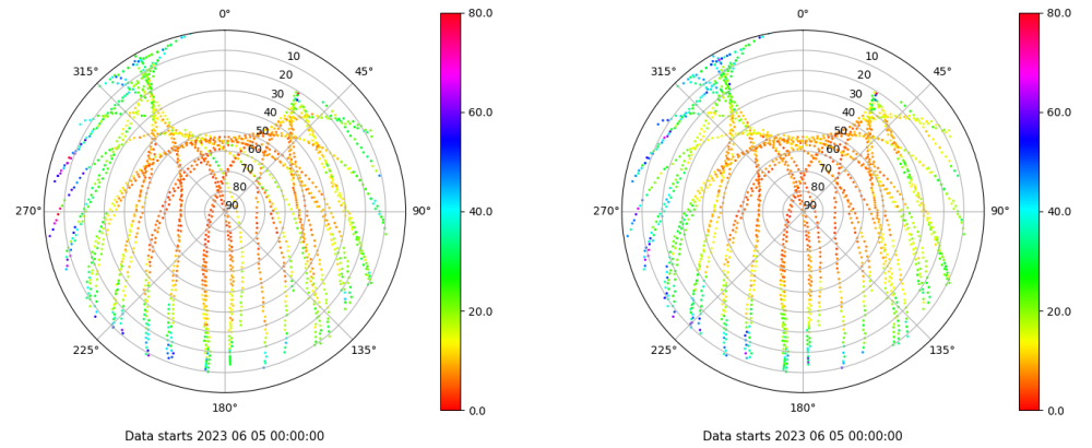
Skyplot for station VICA. Parameter M1C Data file VICA00ESP_R_2023156.xtr Skyplot for station VICA. Parameter M2P Data file VICA00ESP_R_2023156.xtr
