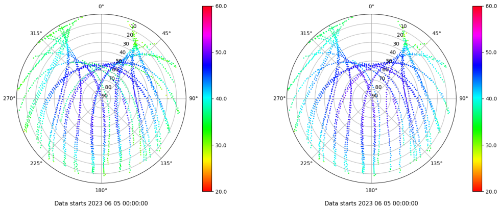
Skyplot for station VICA. Signal to Noise S1C Data file VICA00ESP_R_2023156.xtr Skyplot for station VICA. Signal to Noise S2P Data file VICA00ESP_R_2023156.xtr
