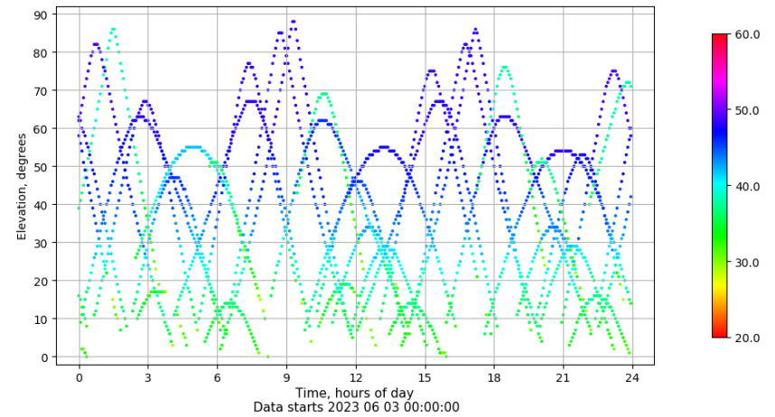
Time-elevation plot for station VICA. Signal to Noise S1C Data file VICA00ESP_R_2023154.xtr
