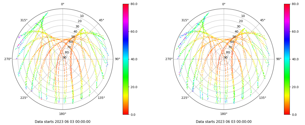
Skyplot for station VICA. Parameter M1C Data file VICA00ESP_R_2023154.xtr Skyplot for station VICA. Parameter M2P Data file VICA00ESP_R_2023154.xtr
