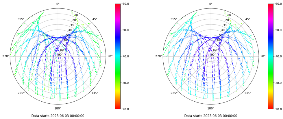
Skyplot for station VICA. Signal to Noise S1C Data file VICA00ESP_R_2023154.xtr Skyplot for station VICA. Signal to Noise S2P Data file VICA00ESP_R_2023154.xtr
