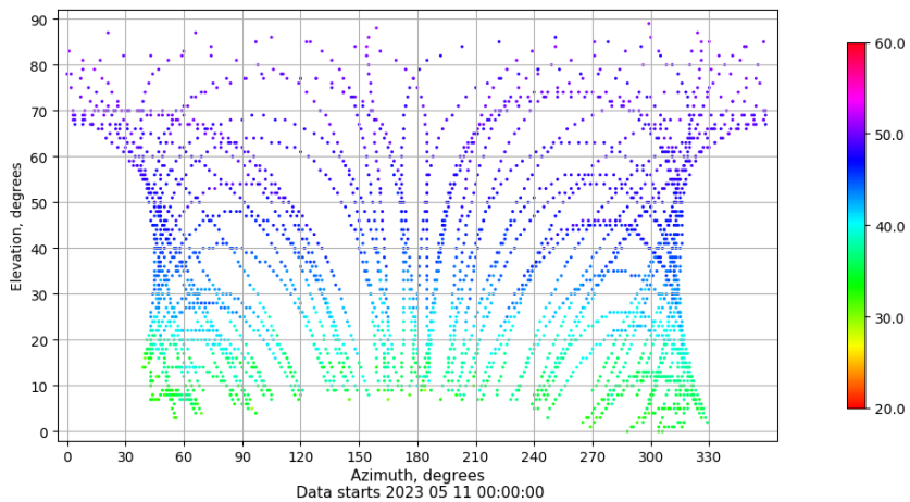
Azimuth-elevation plot for station VICA. Signal to Noise S1C Data file VICA00ESP_R_2023131.xtr
