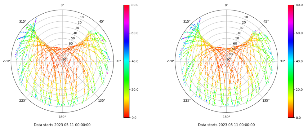
Skyplot for station VICA. Parameter M1C Data file VICA00ESP_R_2023131.xtr Skyplot for station VICA. Parameter M2W Data file VICA00ESP_R_2023131.xtr
