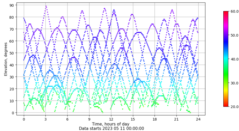
Time-elevation plot for station VICA. Signal to Noise S1C Data file VICA00ESP_R_2023131.xtr
