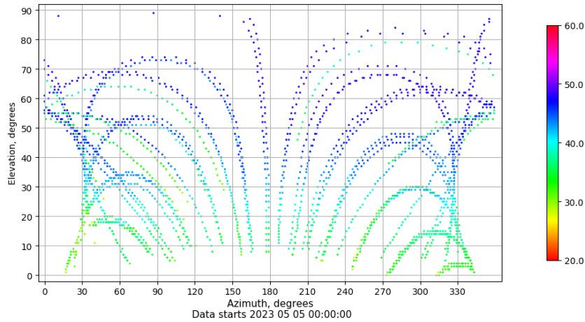
Azimuth-elevation plot for station VICA. Signal to Noise S1C Data file VICA00ESP_R_2023125.xtr
