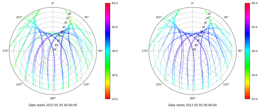
Skyplot for station VICA. Signal to Noise S1C Data file VICA00ESP_R_2023125.xtr Skyplot for station VICA. Signal to Noise S2P Data file VICA00ESP_R_2023125.xtr
