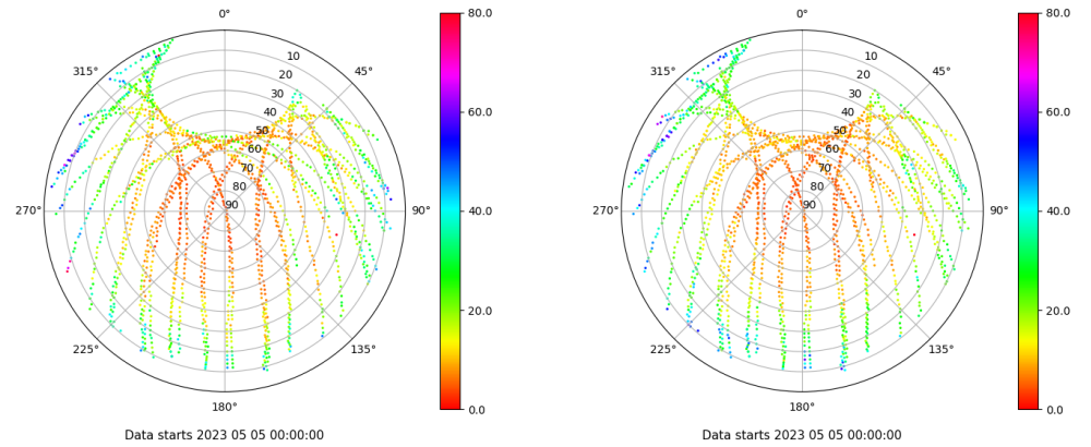
Skyplot for station VICA. Parameter M1C Data file VICA00ESP_R_2023125.xtr Skyplot for station VICA. Parameter M2P Data file VICA00ESP_R_2023125.xtr
