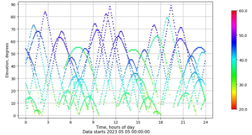
Time-elevation plot for station VICA. Signal to Noise S1C Data file VICA00ESP_R_2023125.xtr
