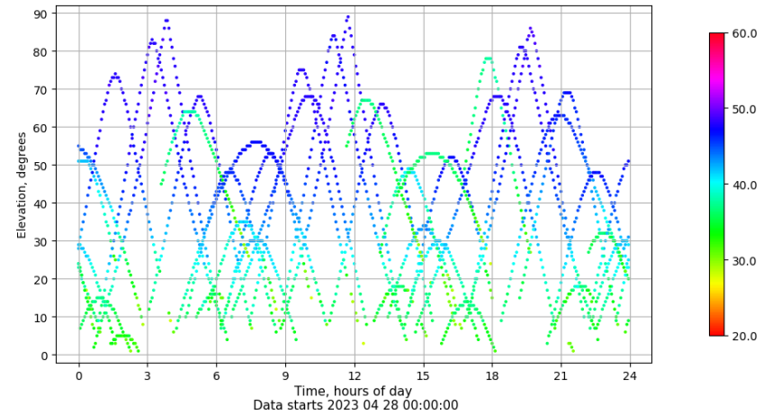
Time-elevation plot for station VICA. Signal to Noise S1C Data file VICA00ESP_R_2023118.xtr
