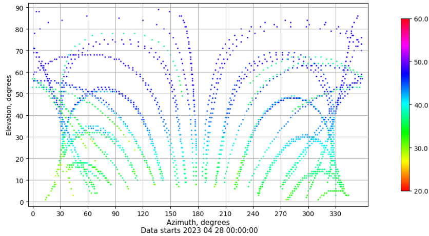
Azimuth-elevation plot for station VICA. Signal to Noise S1C Data file VICA00ESP_R_2023118.xtr
