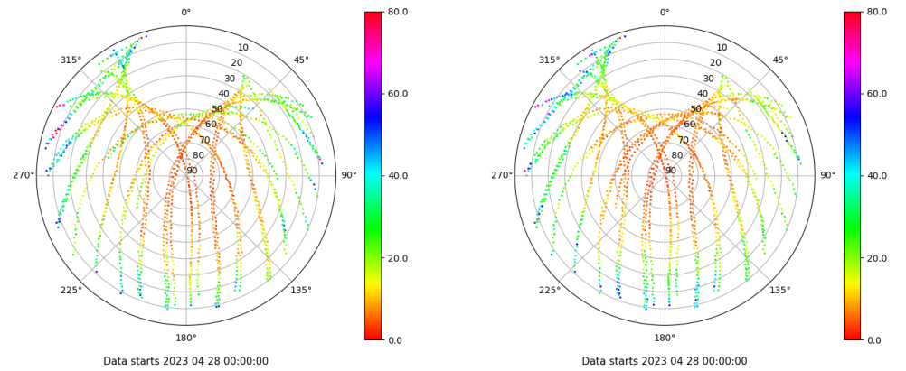
Skyplot for station VICA. Parameter M1C Data file VICA00ESP_R_2023118.xtr Skyplot for station VICA. Parameter M2P Data file VICA00ESP_R_2023118.xtr
