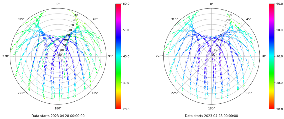
Skyplot for station VICA. Signal to Noise S1C Data file VICA00ESP_R_2023118.xtr Skyplot for station VICA. Signal to Noise S2P Data file VICA00ESP_R_2023118.xtr
