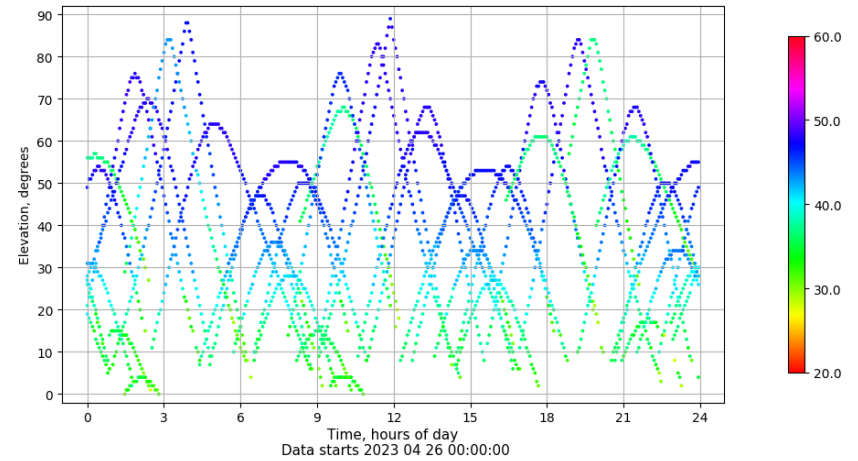
Time-elevation plot for station VICA. Signal to Noise S1C Data file VICA00ESP_R_2023116.xtr
