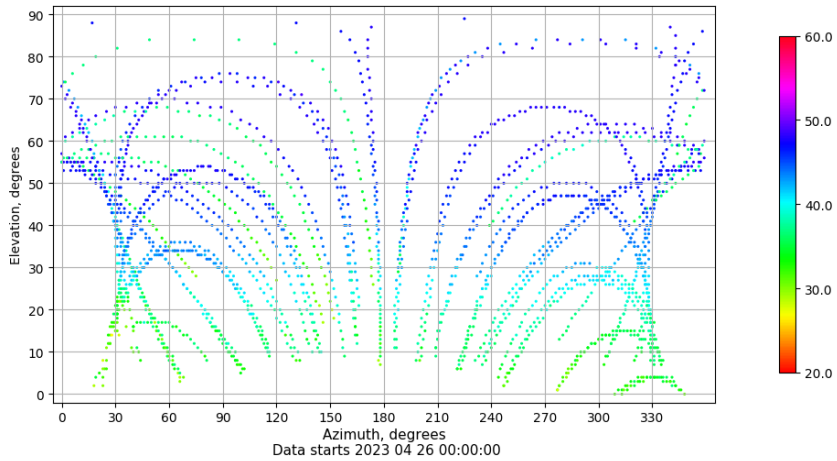
Azimuth-elevation plot for station VICA. Signal to Noise S1C Data file VICA00ESP_R_2023116.xtr
