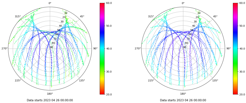
Skyplot for station VICA. Signal to Noise S1C Data file VICA00ESP_R_2023116.xtr Skyplot for station VICA. Signal to Noise S2P Data file VICA00ESP_R_2023116.xtr
