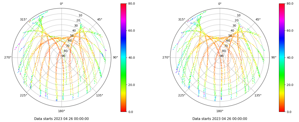
Skyplot for station VICA. Parameter M1C Data file VICA00ESP_R_2023116.xtr Skyplot for station VICA. Parameter M2P Data file VICA00ESP_R_2023116.xtr
