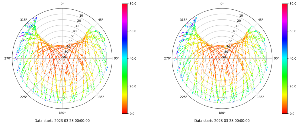
Skyplot for station VICA. Parameter M1C Data file VICA00ESP_R_2023087.xtr Skyplot for station VICA. Parameter M2W Data file VICA00ESP_R_2023087.xtr
