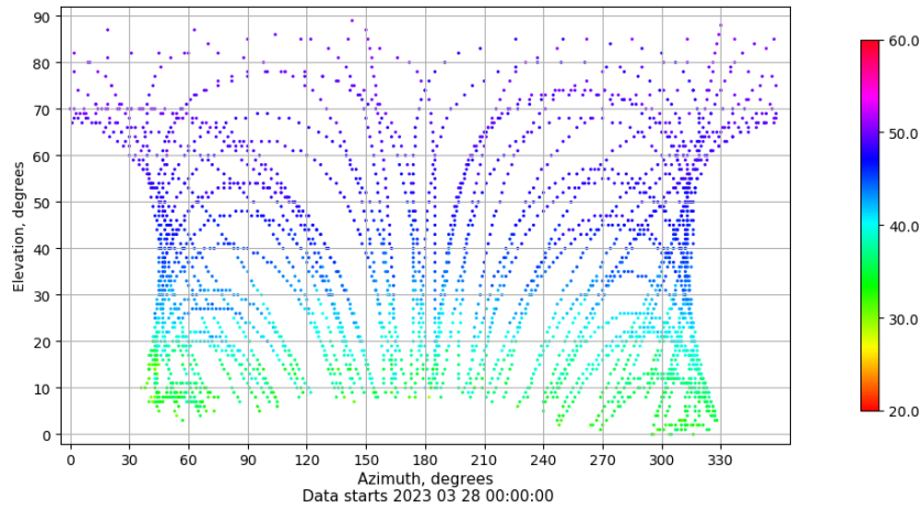
Azimuth-elevation plot for station VICA. Signal to Noise S1C Data file VICA00ESP_R_2023087.xtr
