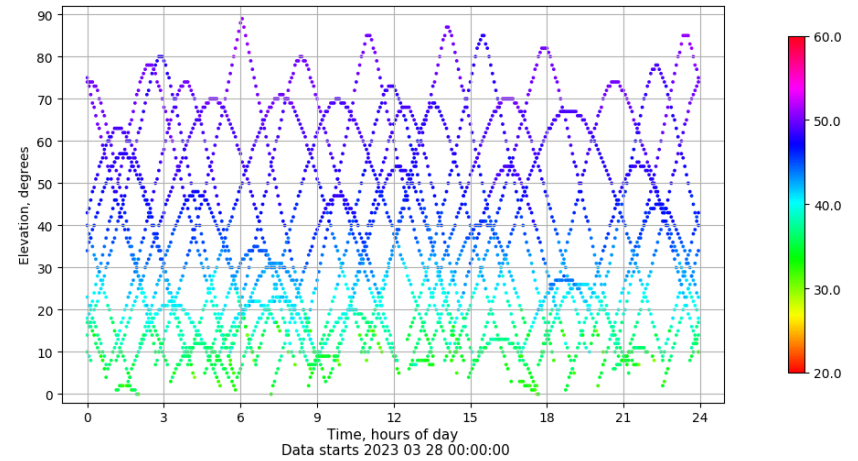
Time-elevation plot for station VICA. Signal to Noise S1C Data file VICA00ESP_R_2023087.xtr
