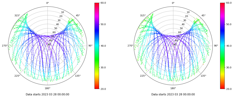
Skyplot for station VICA. Signal to Noise S1C Data file VICA00ESP_R_2023087.xtr Skyplot for station VICA. Signal to Noise S2W Data file VICA00ESP_R_2023087.xtr
