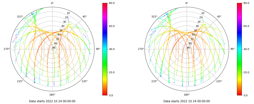
Skyplot for station VICA. Parameter M1C Data file VICA00ESP_R_2022297.xtr Skyplot for station VICA. Parameter M2P Data file VICA00ESP_R_2022297.xtr
