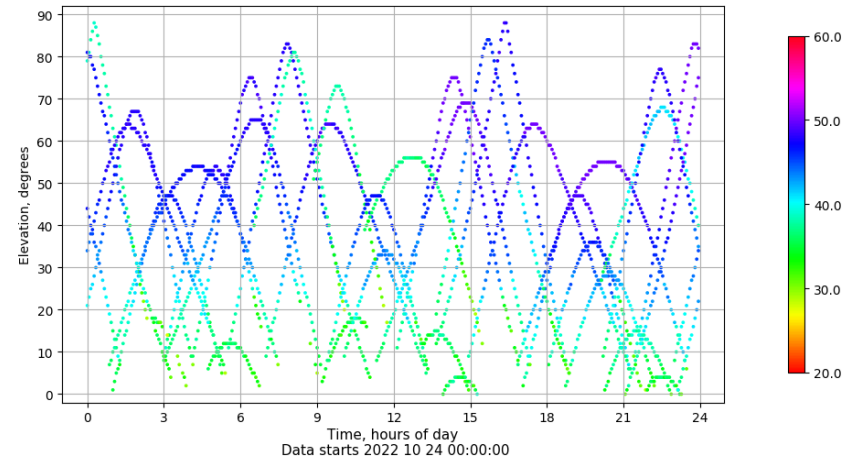
Time-elevation plot for station VICA. Signal to Noise S1C Data file VICA00ESP_R_2022297.xtr
