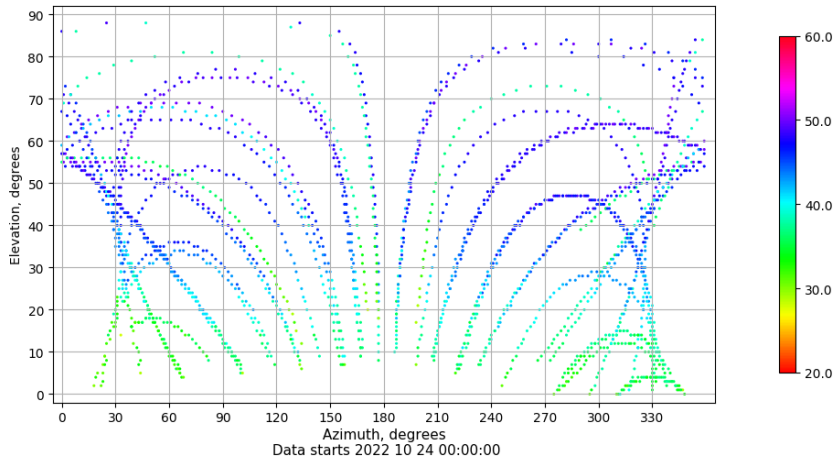
Azimuth-elevation plot for station VICA. Signal to Noise S1C Data file VICA00ESP_R_2022297.xtr
