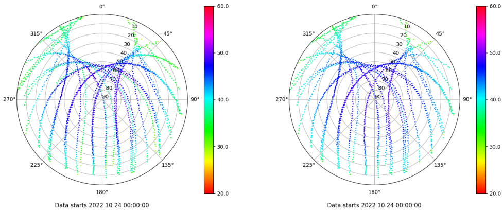
Skyplot for station VICA. Signal to Noise S1C Data file VICA00ESP_R_2022297.xtr Skyplot for station VICA. Signal to Noise S2P Data file VICA00ESP_R_2022297.xtr
