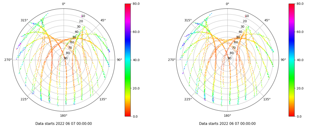
Skyplot for station VICA. Parameter M1C Data file VICA00ESP_R_2022158.xtr Skyplot for station VICA. Parameter M2P Data file VICA00ESP_R_2022158.xtr
