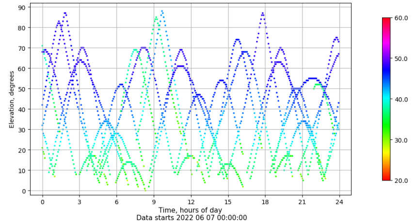
Time-elevation plot for station VICA. Signal to Noise S1C Data file VICA00ESP_R_2022158.xtr
