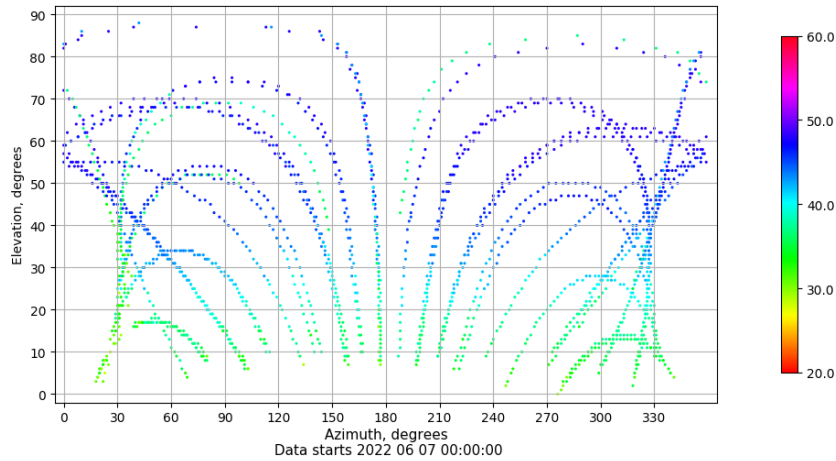
Azimuth-elevation plot for station VICA. Signal to Noise S1C Data file VICA00ESP_R_2022158.xtr
