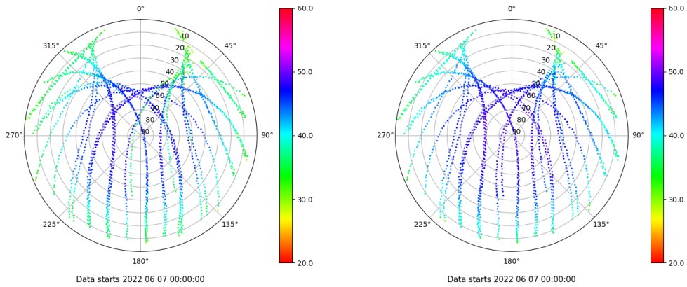
Skyplot for station VICA. Signal to Noise S1C Data file VICA00ESP_R_2022158.xtr Skyplot for station VICA. Signal to Noise S2P Data file VICA00ESP_R_2022158.xtr
