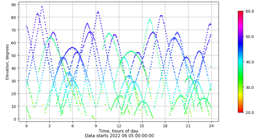
Time-elevation plot for station VICA. Signal to Noise S1C Data file VICA00ESP_R_2022156.xtr
