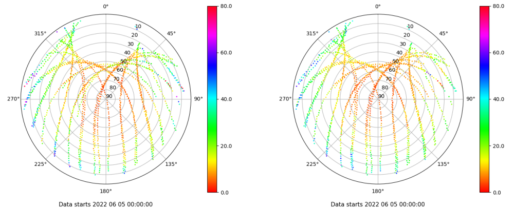
Skyplot for station VICA. Parameter M1C Data file VICA00ESP_R_2022156.xtr Skyplot for station VICA. Parameter M2P Data file VICA00ESP_R_2022156.xtr
