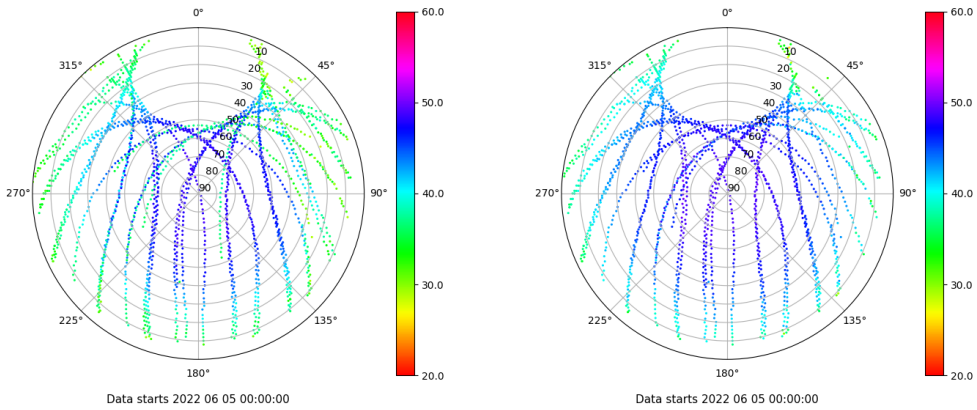
Skyplot for station VICA. Signal to Noise S1C Data file VICA00ESP_R_2022156.xtr Skyplot for station VICA. Signal to Noise S2P Data file VICA00ESP_R_2022156.xtr
