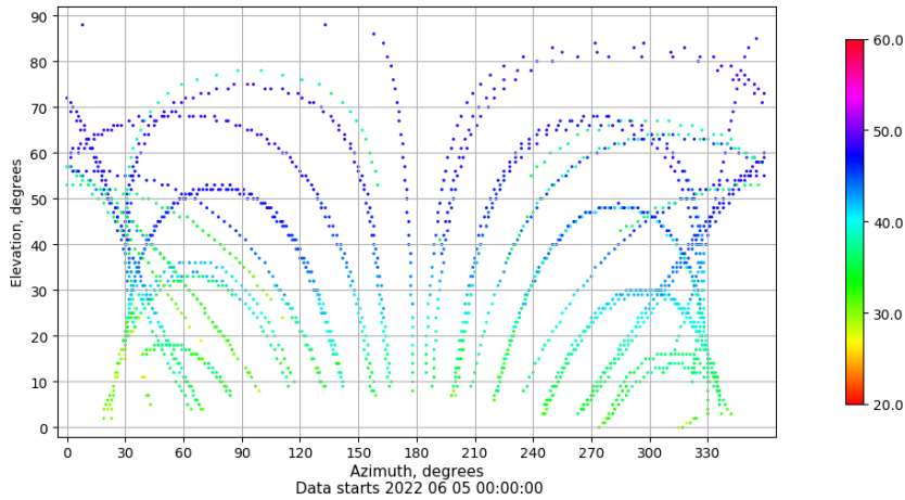
Azimuth-elevation plot for station VICA. Signal to Noise S1C Data file VICA00ESP_R_2022156.xtr
