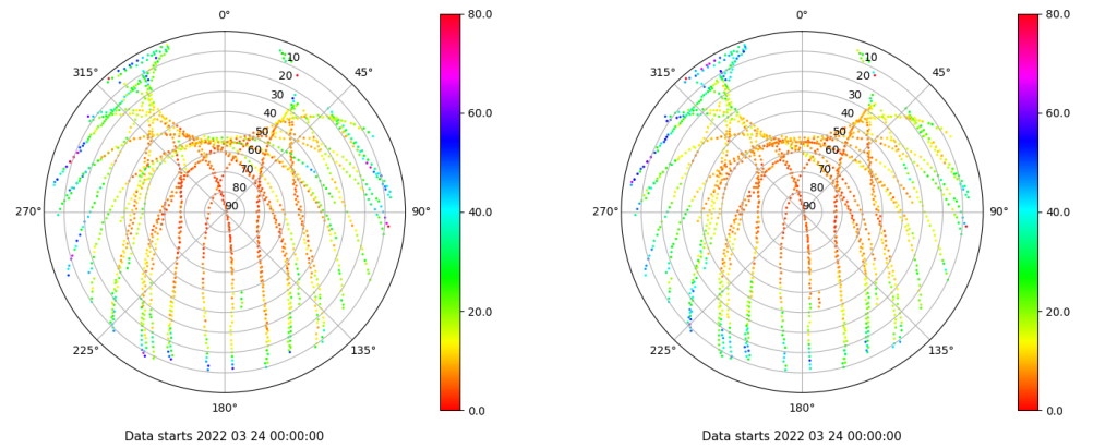
Skyplot for station VICA. Parameter M1C Data file VICA00ESP_R_2022083.xtr Skyplot for station VICA. Parameter M2P Data file VICA00ESP_R_2022083.xtr
