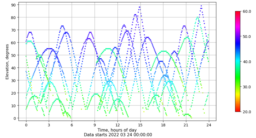
Time-elevation plot for station VICA. Signal to Noise S1C Data file VICA00ESP_R_2022083.xtr
