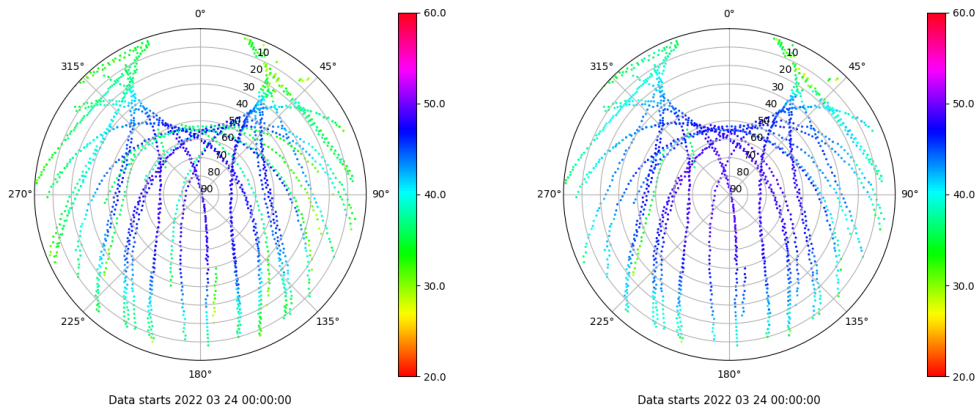
Skyplot for station VICA. Signal to Noise S1C Data file VICA00ESP_R_2022083.xtr Skyplot for station VICA. Signal to Noise S2P Data file VICA00ESP_R_2022083.xtr
