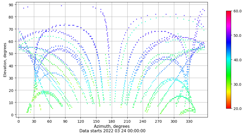
Azimuth-elevation plot for station VICA. Signal to Noise S1C Data file VICA00ESP_R_2022083.xtr
