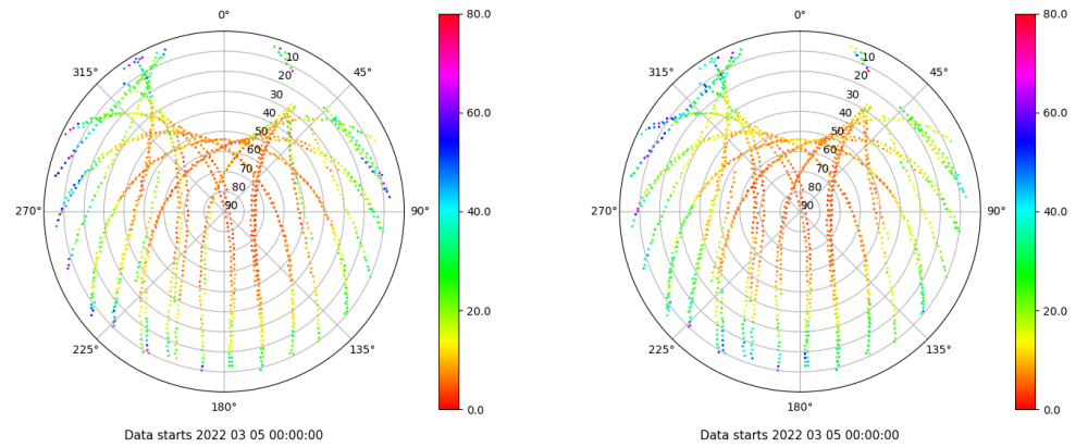
Skyplot for station VICA. Parameter M1C Data file VICA00ESP_R_2022064.xtr Skyplot for station VICA. Parameter M2P Data file VICA00ESP_R_2022064.xtr
