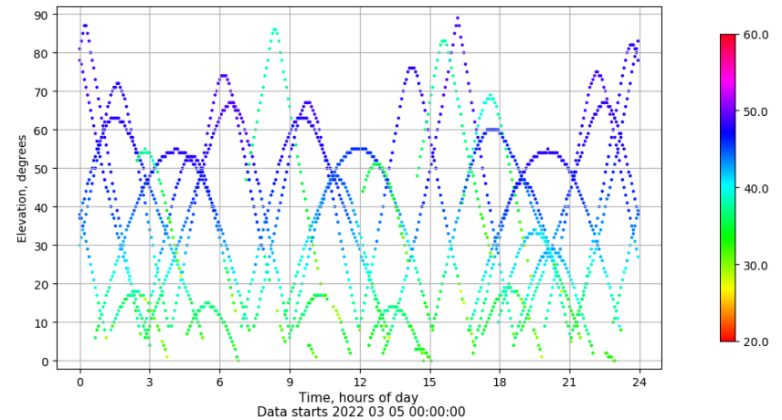
Time-elevation plot for station VICA. Signal to Noise S1C Data file VICA00ESP_R_2022064.xtr
