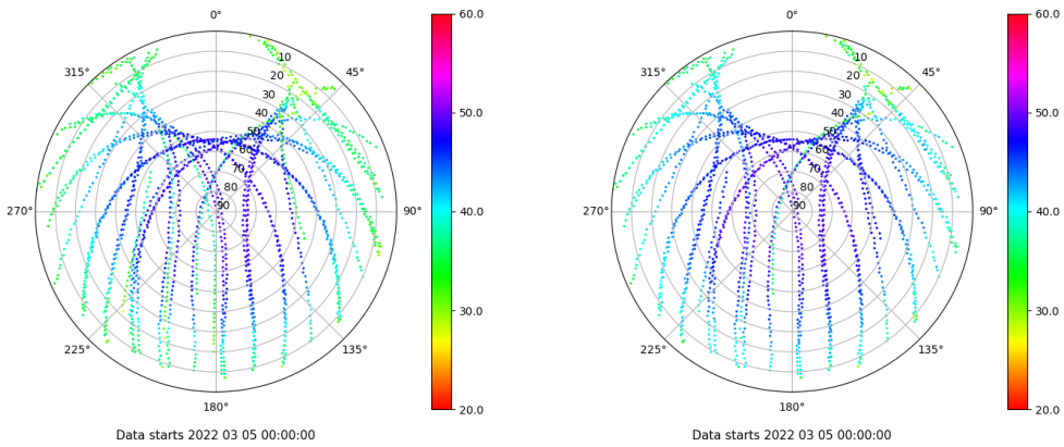
Skyplot for station VICA. Signal to Noise S1C Data file VICA00ESP_R_2022064.xtr Skyplot for station VICA. Signal to Noise S2P Data file VICA00ESP_R_2022064.xtr
