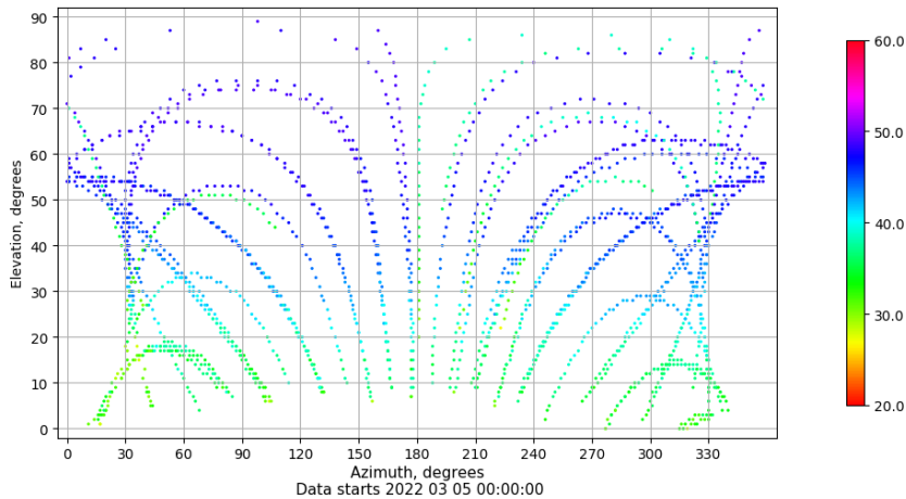
Azimuth-elevation plot for station VICA. Signal to Noise S1C Data file VICA00ESP_R_2022064.xtr
