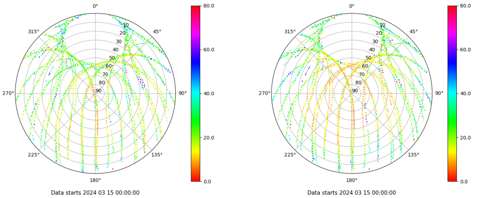
Skyplot for station VALE. Parameter M1C Data file VALE00ESP_R_2024075.xtr Skyplot for station VALE. Parameter M2P Data file VALE00ESP_R_2024075.xtr
