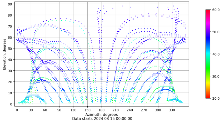
Azimuth-elevation plot for station VALE. Signal to Noise S1C Data file VALE00ESP_R_2024075.xtr
