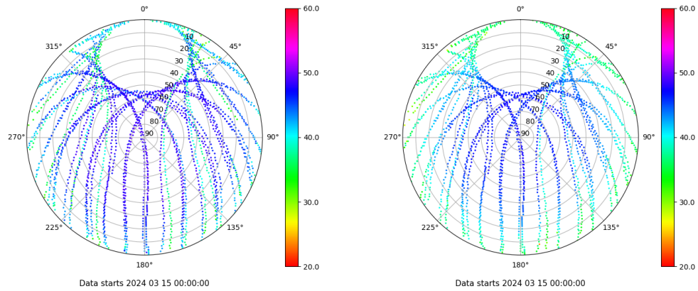
Skyplot for station VALE. Signal to Noise S1C Data file VALE00ESP_R_2024075.xtr Skyplot for station VALE. Signal to Noise S2P Data file VALE00ESP_R_2024075.xtr
