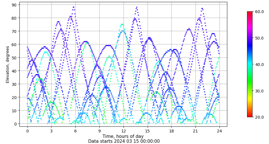
Time-elevation plot for station VALE. Signal to Noise S1C Data file VALE00ESP_R_2024075.xtr
