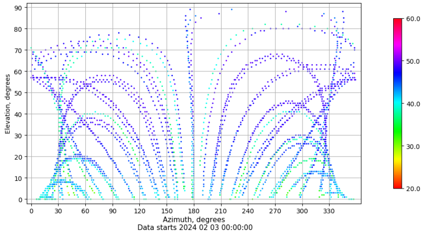
Azimuth-elevation plot for station VALE. Signal to Noise S1C Data file VALE00ESP_R_2024034.xtr
