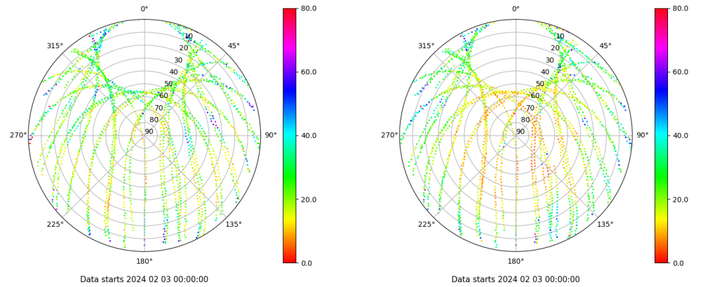
Skyplot for station VALE. Parameter M1C Data file VALE00ESP_R_2024034.xtr Skyplot for station VALE. Parameter M2P Data file VALE00ESP_R_2024034.xtr
