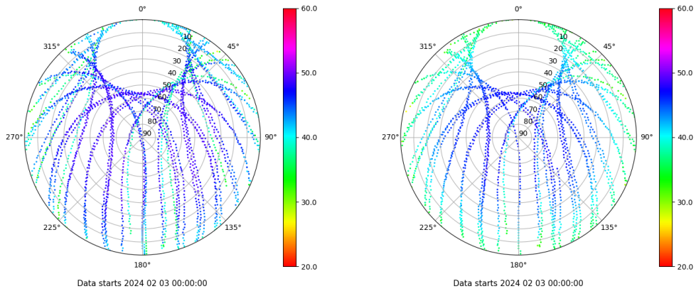
Skyplot for station VALE. Signal to Noise S1C Data file VALE00ESP_R_2024034.xtr Skyplot for station VALE. Signal to Noise S2P Data file VALE00ESP_R_2024034.xtr
