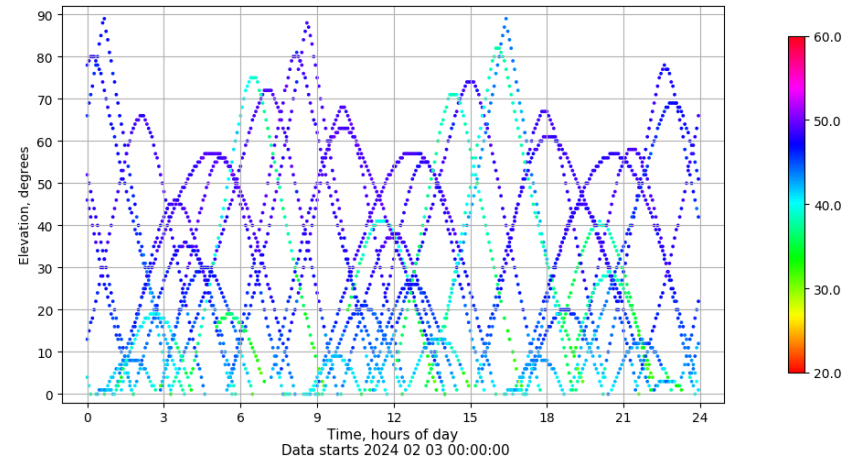
Time-elevation plot for station VALE. Signal to Noise S1C Data file VALE00ESP_R_2024034.xtr
