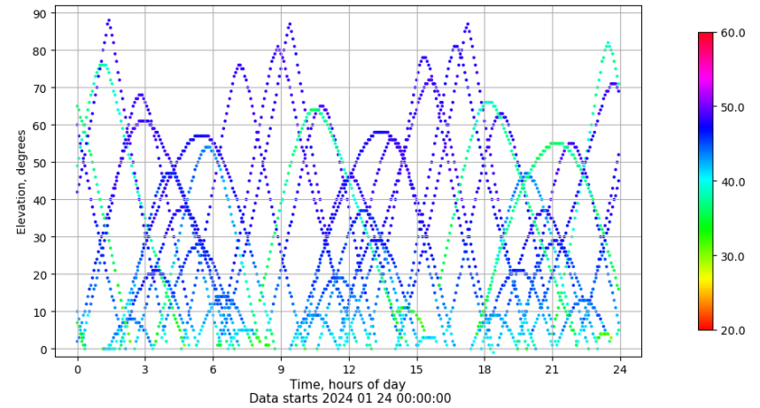
Time-elevation plot for station VALE. Signal to Noise S1C Data file VALE00ESP_R_2024024.xtr
