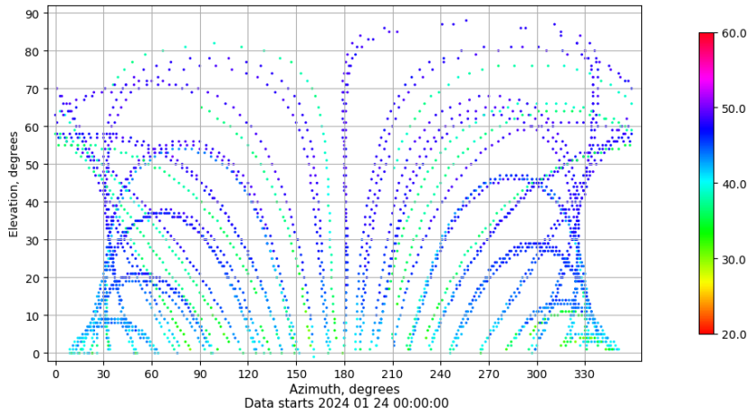
Azimuth-elevation plot for station VALE. Signal to Noise S1C Data file VALE00ESP_R_2024024.xtr
