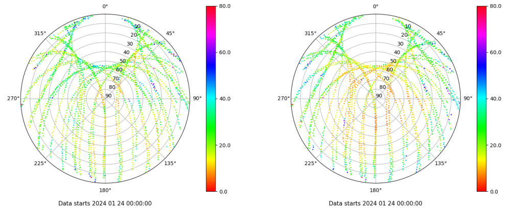
Skyplot for station VALE. Parameter M1C Data file VALE00ESP_R_2024024.xtr Skyplot for station VALE. Parameter M2P Data file VALE00ESP_R_2024024.xtr
