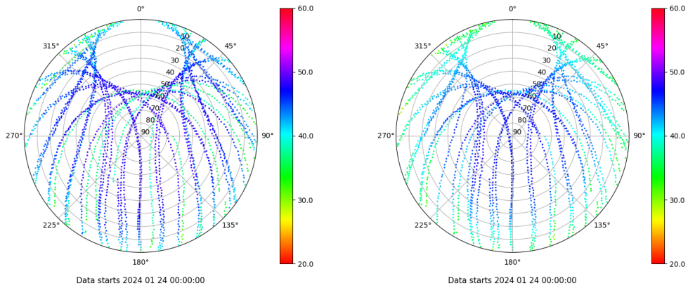
Skyplot for station VALE. Signal to Noise S1C Data file VALE00ESP_R_2024024.xtr Skyplot for station VALE. Signal to Noise S2P Data file VALE00ESP_R_2024024.xtr
