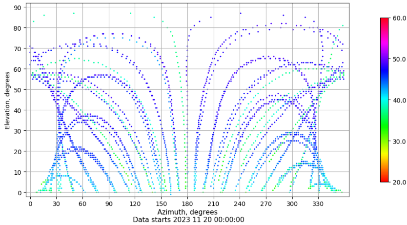
Azimuth-elevation plot for station VALE. Signal to Noise S1C Data file VALE00ESP_R_2023324.xtr
