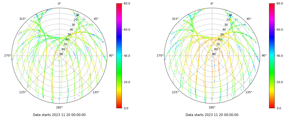
Skyplot for station VALE. Parameter M1C Data file VALE00ESP_R_2023324.xtr Skyplot for station VALE. Parameter M2P Data file VALE00ESP_R_2023324.xtr
