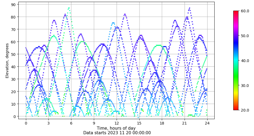
Time-elevation plot for station VALE. Signal to Noise S1C Data file VALE00ESP_R_2023324.xtr
