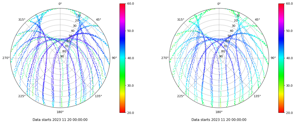
Skyplot for station VALE. Signal to Noise S1C Data file VALE00ESP_R_2023324.xtr Skyplot for station VALE. Signal to Noise S2P Data file VALE00ESP_R_2023324.xtr
