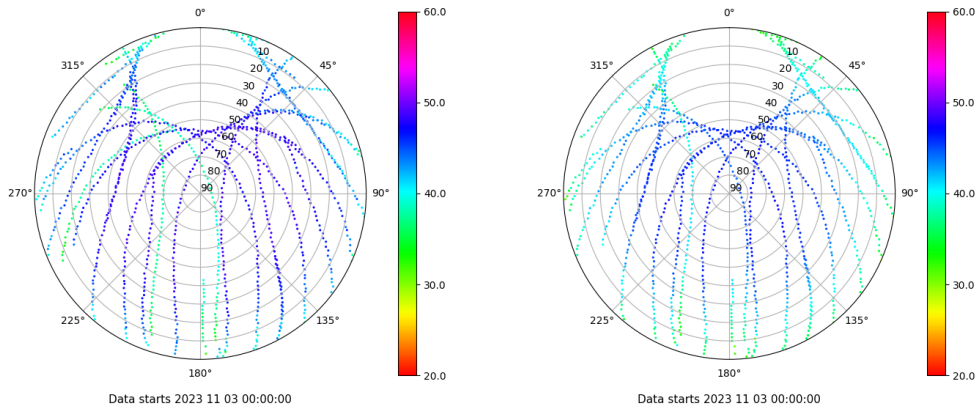
Skyplot for station VALE. Signal to Noise S1C Data file VALE00ESP_R_2023307.xtr Skyplot for station VALE. Signal to Noise S2P Data file VALE00ESP_R_2023307.xtr
