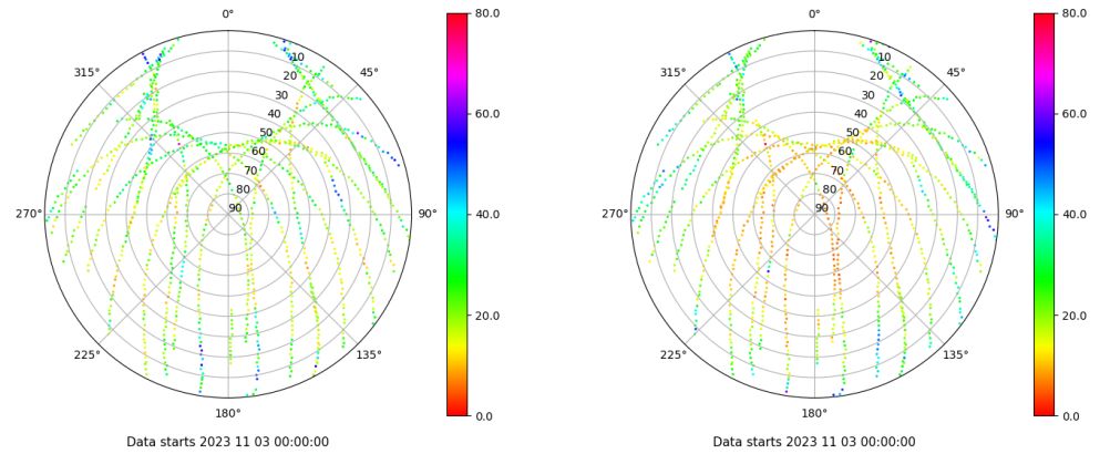
Skyplot for station VALE. Parameter M1C Data file VALE00ESP_R_2023307.xtr Skyplot for station VALE. Parameter M2P Data file VALE00ESP_R_2023307.xtr
