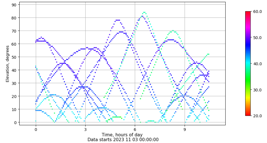
Time-elevation plot for station VALE. Signal to Noise S1C Data file VALE00ESP_R_2023307.xtr
