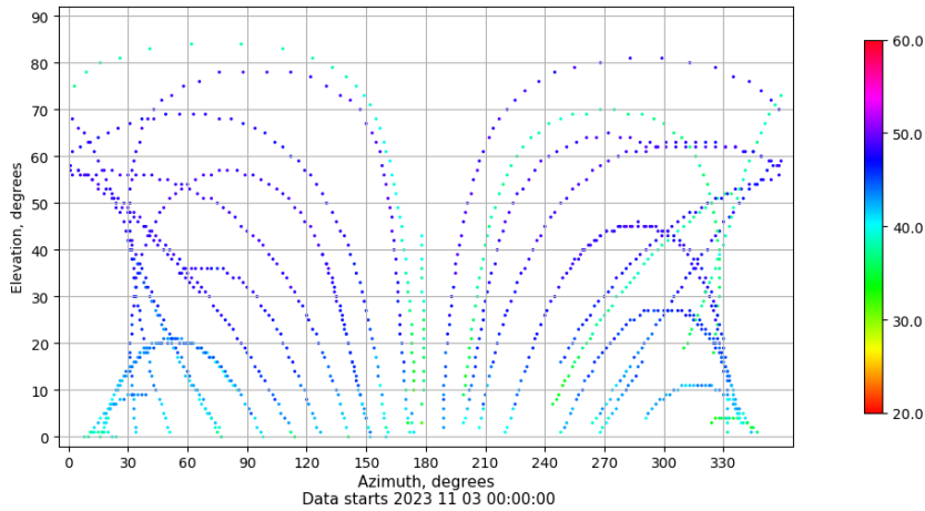
Azimuth-elevation plot for station VALE. Signal to Noise S1C Data file VALE00ESP_R_2023307.xtr
