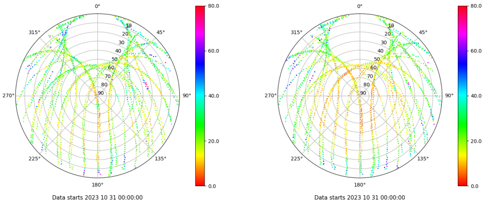
Skyplot for station VALE. Parameter M1C Data file VALE00ESP_R_2023304.xtr Skyplot for station VALE. Parameter M2P Data file VALE00ESP_R_2023304.xtr
