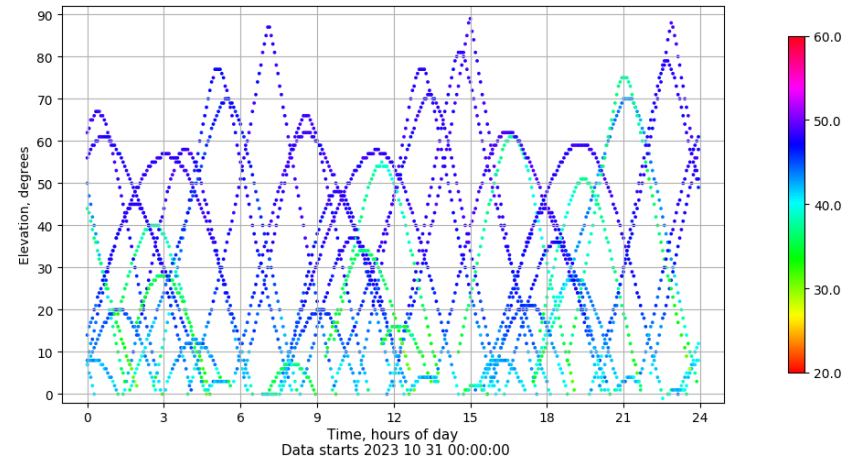
Time-elevation plot for station VALE. Signal to Noise S1C Data file VALE00ESP_R_2023304.xtr
