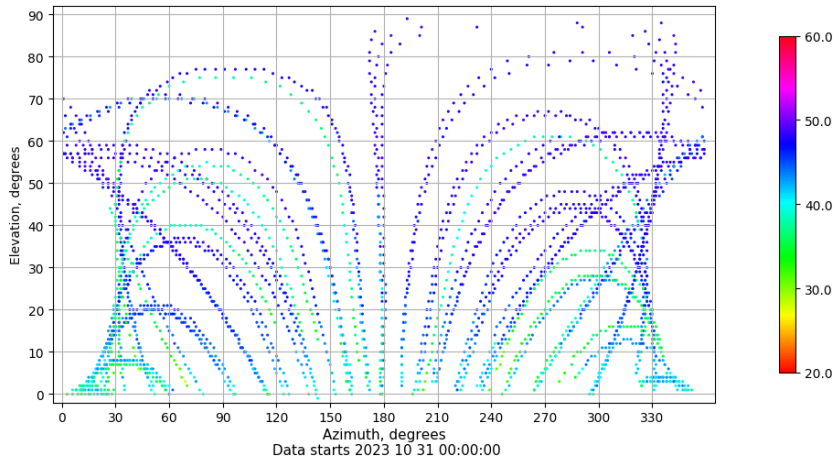
Azimuth-elevation plot for station VALE. Signal to Noise S1C Data file VALE00ESP_R_2023304.xtr
