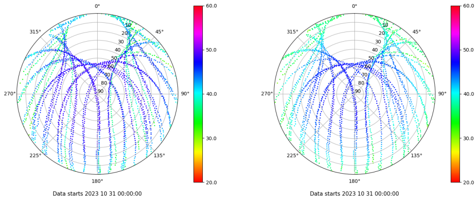
Skyplot for station VALE. Signal to Noise S1C Data file VALE00ESP_R_2023304.xtr Skyplot for station VALE. Signal to Noise S2P Data file VALE00ESP_R_2023304.xtr
