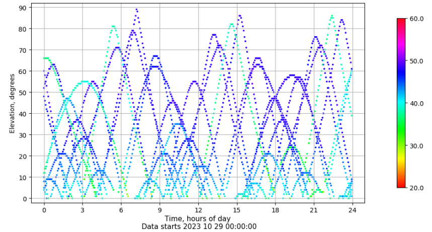
Time-elevation plot for station VALE. Signal to Noise S1C Data file VALE00ESP_R_2023302.xtr
