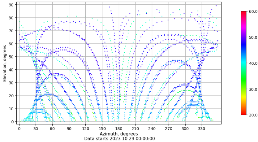
Azimuth-elevation plot for station VALE. Signal to Noise S1C Data file VALE00ESP_R_2023302.xtr
