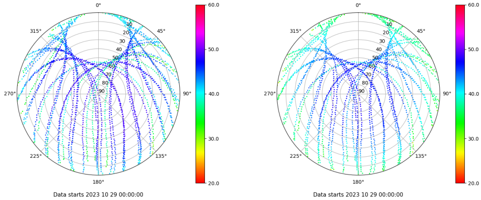
Skyplot for station VALE. Signal to Noise S1C Data file VALE00ESP_R_2023302.xtr Skyplot for station VALE. Signal to Noise S2P Data file VALE00ESP_R_2023302.xtr
