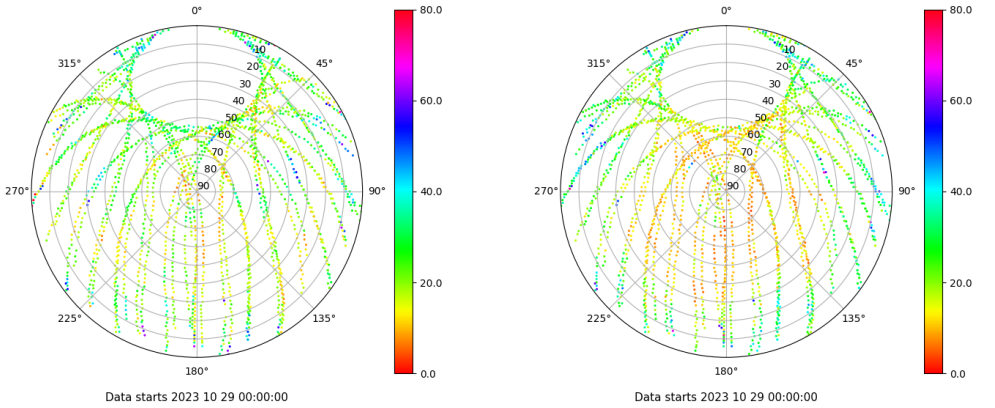
Skyplot for station VALE. Parameter M1C Data file VALE00ESP_R_2023302.xtr Skyplot for station VALE. Parameter M2P Data file VALE00ESP_R_2023302.xtr
