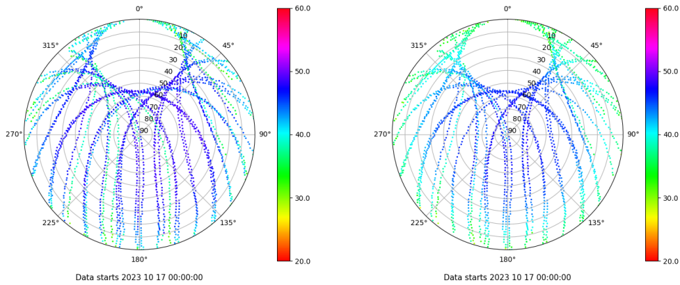
Skyplot for station VALE. Signal to Noise S1C Data file VALE00ESP_R_2023290.xtr Skyplot for station VALE. Signal to Noise S2P Data file VALE00ESP_R_2023290.xtr
