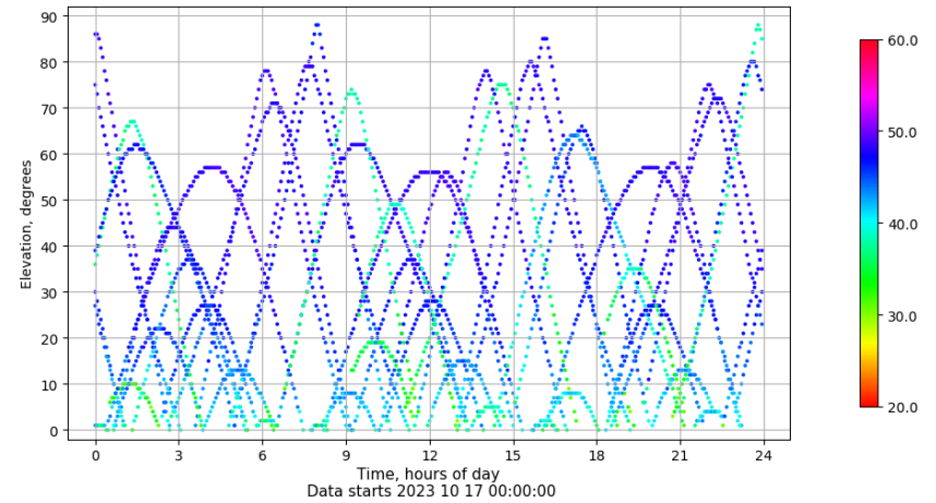
Time-elevation plot for station VALE. Signal to Noise S1C Data file VALE00ESP_R_2023290.xtr
