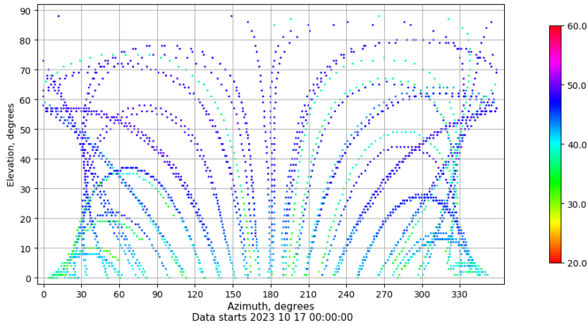
Azimuth-elevation plot for station VALE. Signal to Noise S1C Data file VALE00ESP_R_2023290.xtr
